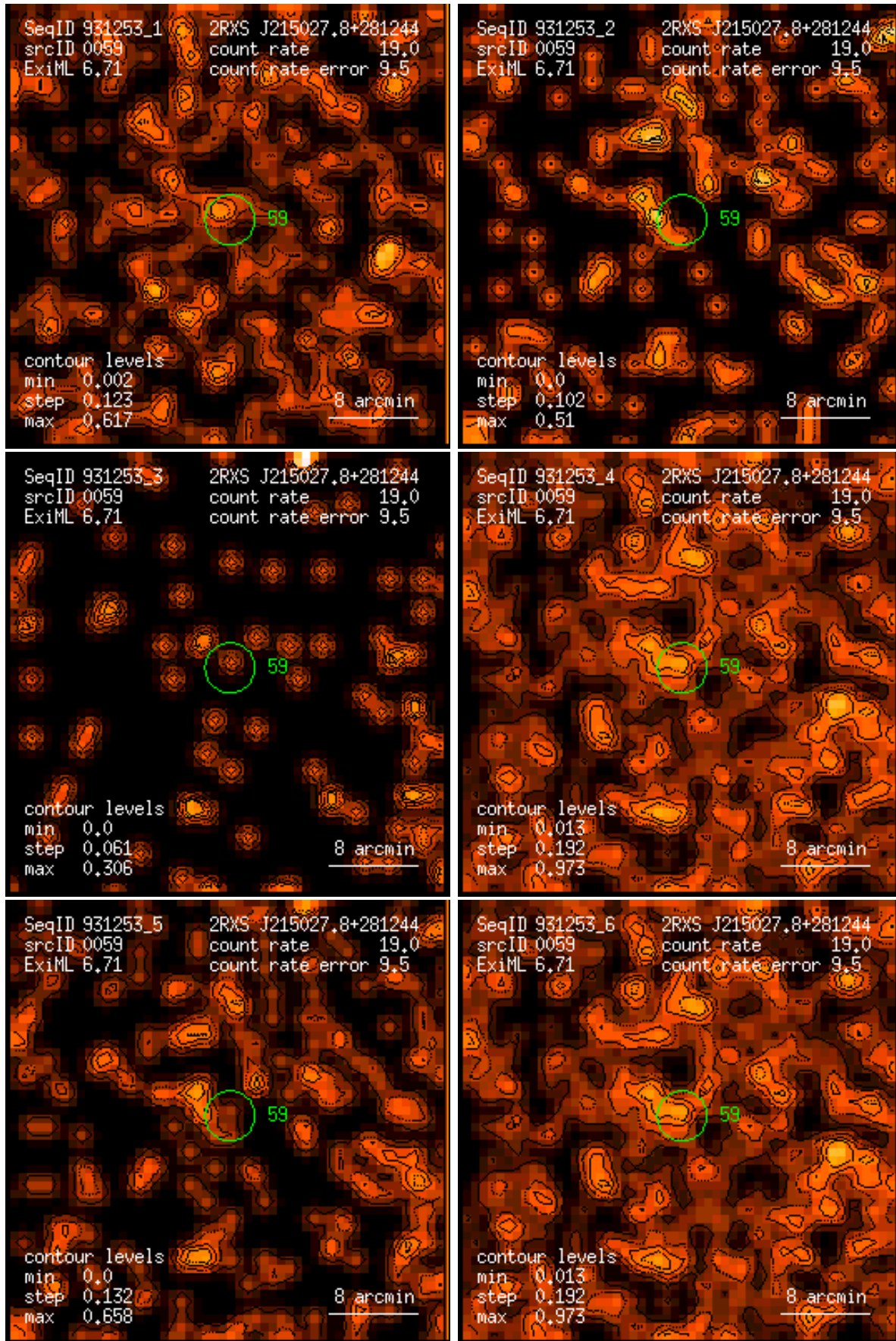
Figure 59: RASS 931253: detection 0059: band rate images, Gaussian filter: (1) PSPC channels 11 – 41, (2) 52 – 90, (3) 91 – 201, (4) 11 – 235, (5) 52 – 201, (6) 11 – 201. Broad band rates in counts/ks. Band rate contour levels in counts/ks/arcmin 2 .
