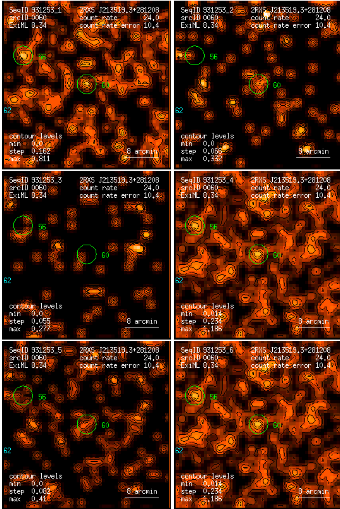
Figure 60: RASS 931253: detection 0060: band rate images, Gaussian filter: (1) PSPC channels 11 – 41, (2) 52 – 90, (3) 91 – 201, (4) 11 – 235, (5) 52 – 201, (6) 11 – 201. Broad band rates in counts/ks. Band rate contour levels in counts/ks/arcmin 2 .
