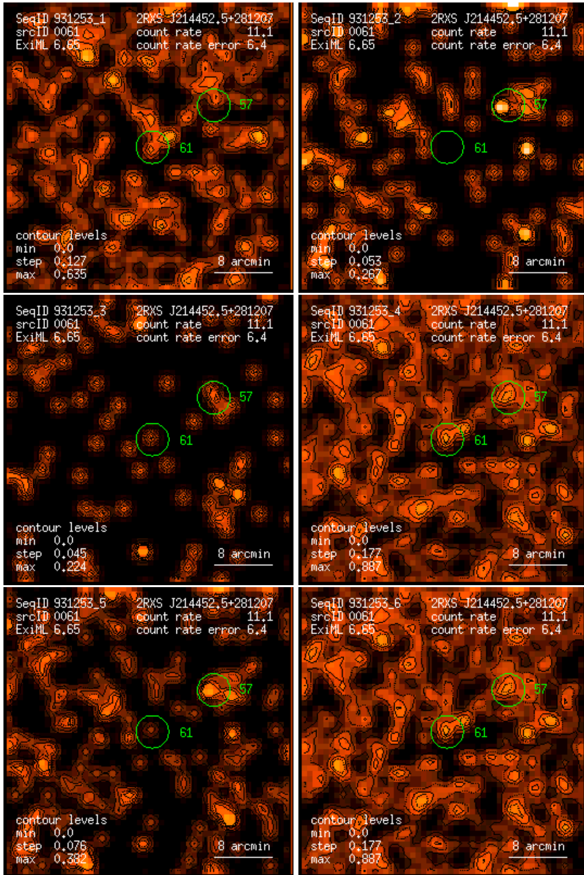
Figure 61: RASS 931253: detection 0061: band rate images, Gaussian filter: (1) PSPC channels 11 – 41, (2) 52 – 90, (3) 91 – 201, (4) 11 – 235, (5) 52 – 201, (6) 11 – 201. Broad band rates in counts/ks. Band rate contour levels in counts/ks/arcmin 2 .
