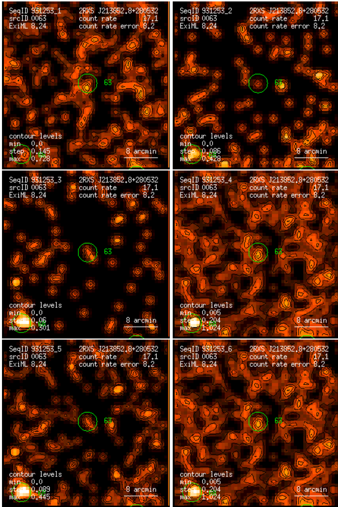
Figure 63: RASS 931253: detection 0063: band rate images, Gaussian filter: (1) PSPC channels 11 – 41, (2) 52 – 90, (3) 91 – 201, (4) 11 – 235, (5) 52 – 201, (6) 11 – 201. Broad band rates in counts/ks. Band rate contour levels in counts/ks/arcmin 2 .
