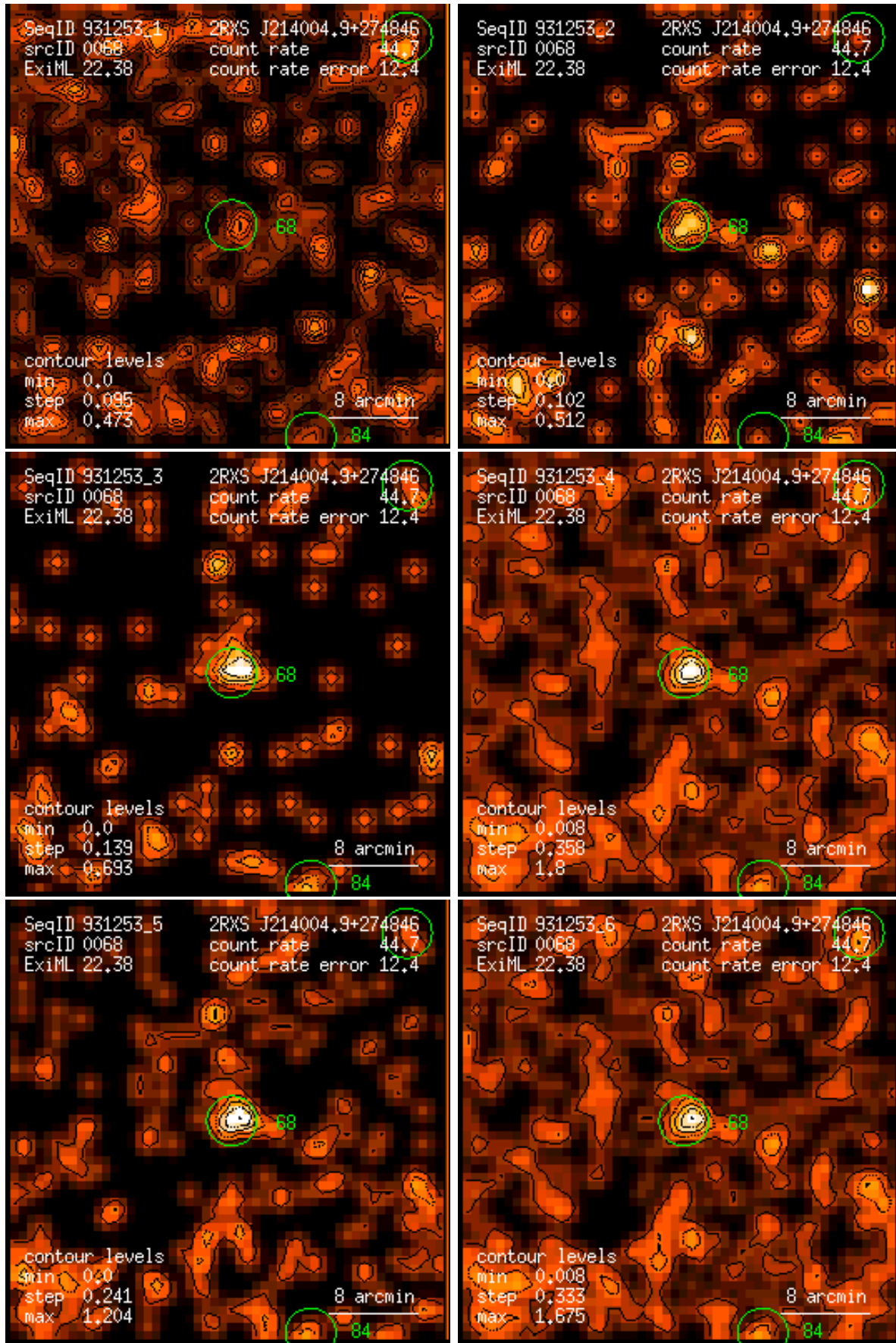
Figure 68: RASS 931253: detection 0068: band rate images, Gaussian filter: (1) PSPC channels 11 – 41, (2) 52 – 90, (3) 91 – 201, (4) 11 – 235, (5) 52 – 201, (6) 11 – 201. Broad band rates in counts/ks. Band rate contour levels in counts/ks/arcmin 2 .
