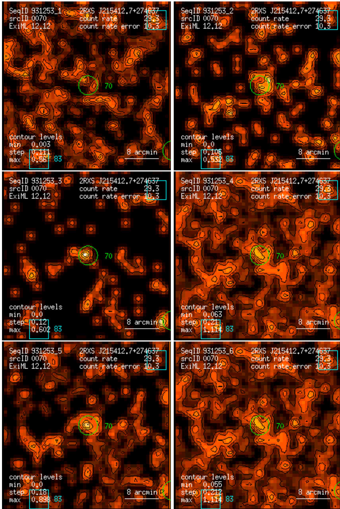
Figure 70: RASS 931253: detection 0070: band rate images, Gaussian filter: (1) PSPC channels 11 – 41, (2) 52 – 90, (3) 91 – 201, (4) 11 – 235, (5) 52 – 201, (6) 11 – 201. Broad band rates in counts/ks. Band rate contour levels in counts/ks/arcmin 2 .
