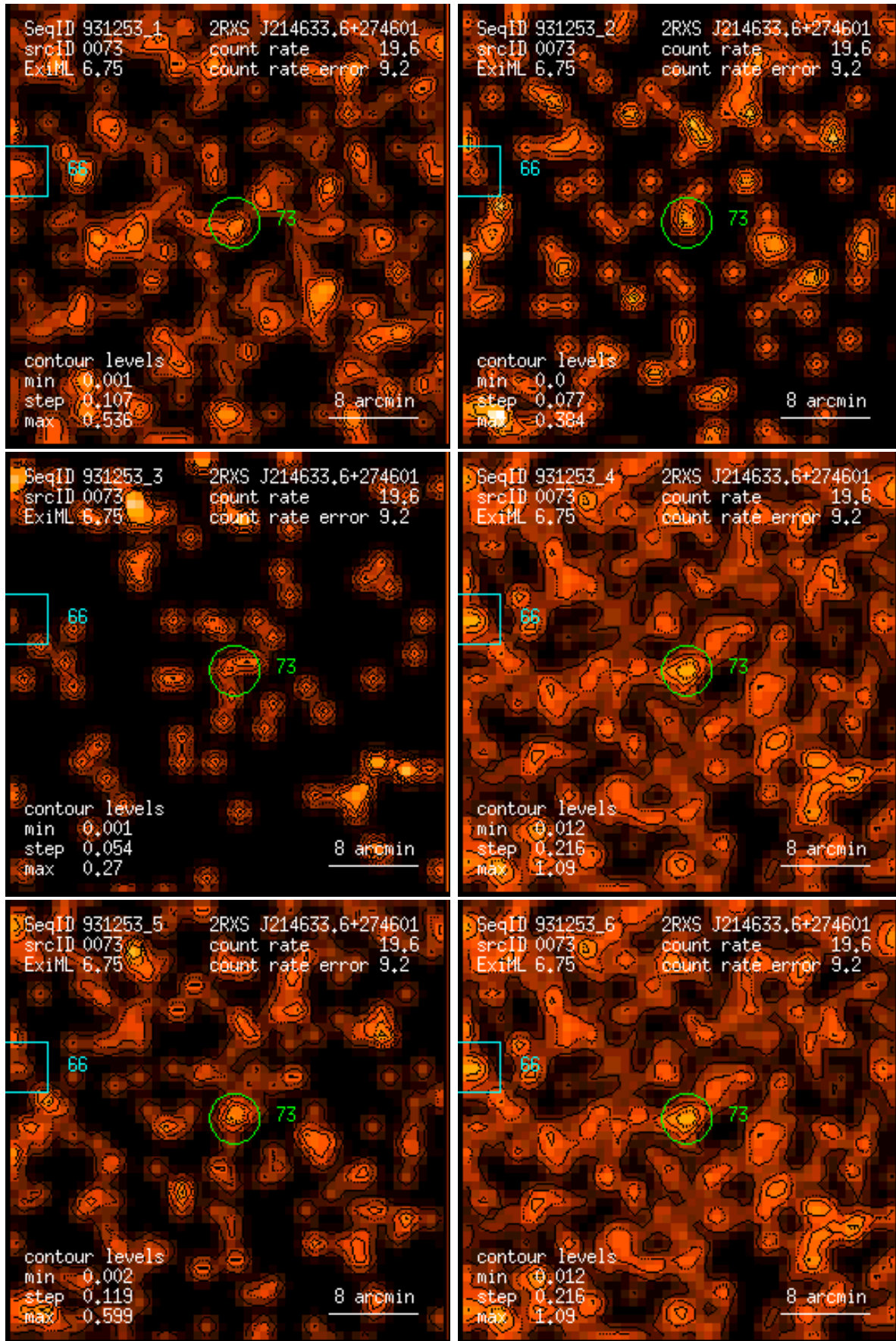
Figure 73: RASS 931253: detection 0073: band rate images, Gaussian filter: (1) PSPC channels 11 – 41, (2) 52 – 90, (3) 91 – 201, (4) 11 – 235, (5) 52 – 201, (6) 11 – 201. Broad band rates in counts/ks. Band rate contour levels in counts/ks/arcmin 2 .
