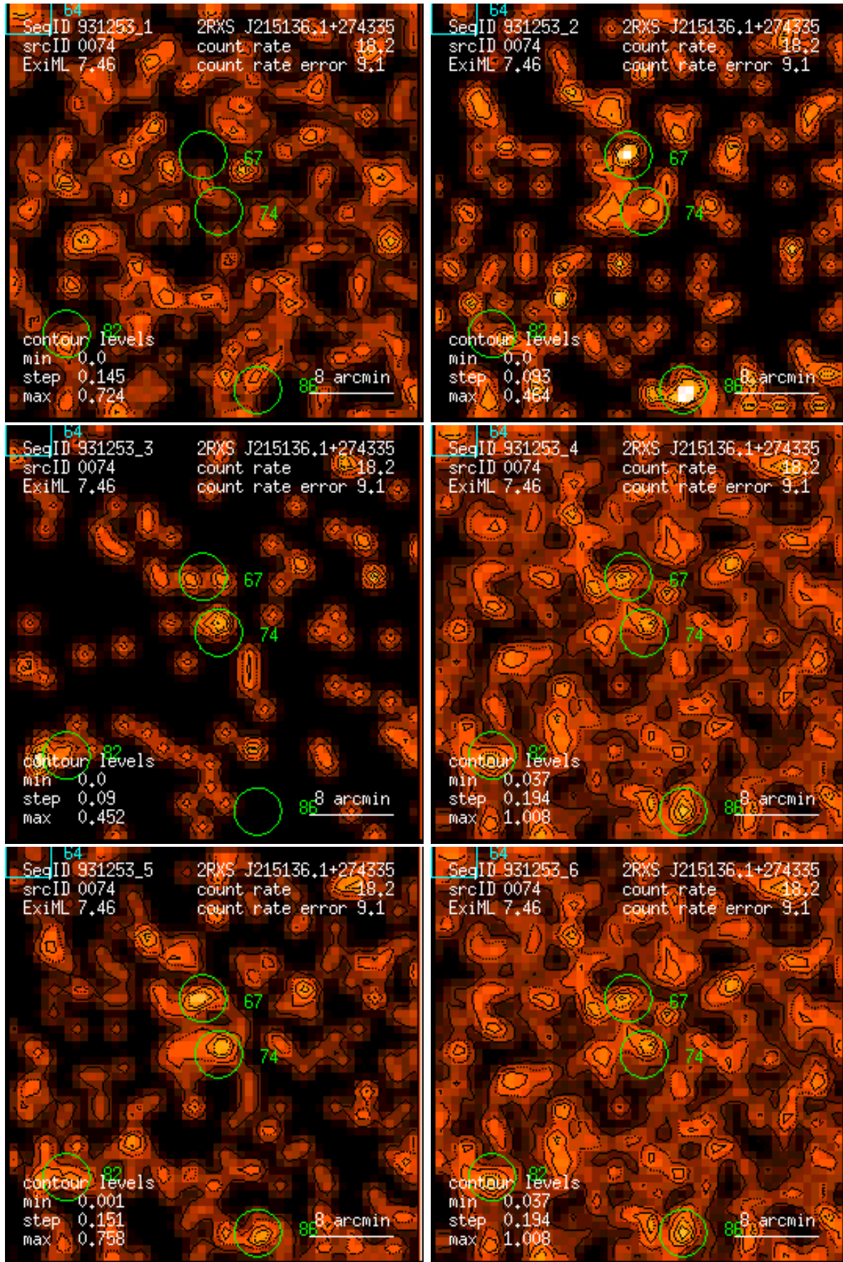
Figure 74: RASS 931253: detection 0074: band rate images, Gaussian filter: (1) PSPC channels 11 – 41, (2) 52 – 90, (3) 91 – 201, (4) 11 – 235, (5) 52 – 201, (6) 11 – 201. Broad band rates in counts/ks. Band rate contour levels in counts/ks/arcmin 2 .
