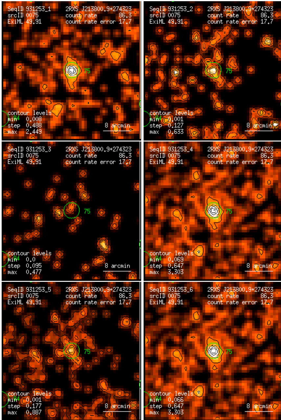
Figure 75: RASS 931253: detection 0075: band rate images, Gaussian filter: (1) PSPC channels 11 – 41, (2) 52 – 90, (3) 91 – 201, (4) 11 – 235, (5) 52 – 201, (6) 11 – 201. Broad band rates in counts/ks. Band rate contour levels in counts/ks/arcmin 2 .
