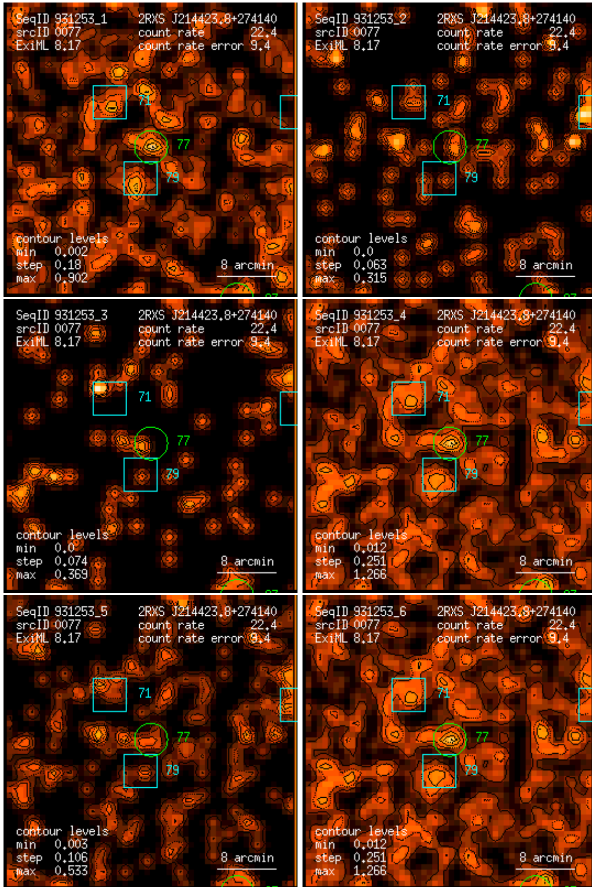
Figure 77: RASS 931253: detection 0077: band rate images, Gaussian filter: (1) PSPC channels 11 – 41, (2) 52 – 90, (3) 91 – 201, (4) 11 – 235, (5) 52 – 201, (6) 11 – 201. Broad band rates in counts/ks. Band rate contour levels in counts/ks/arcmin 2 .
