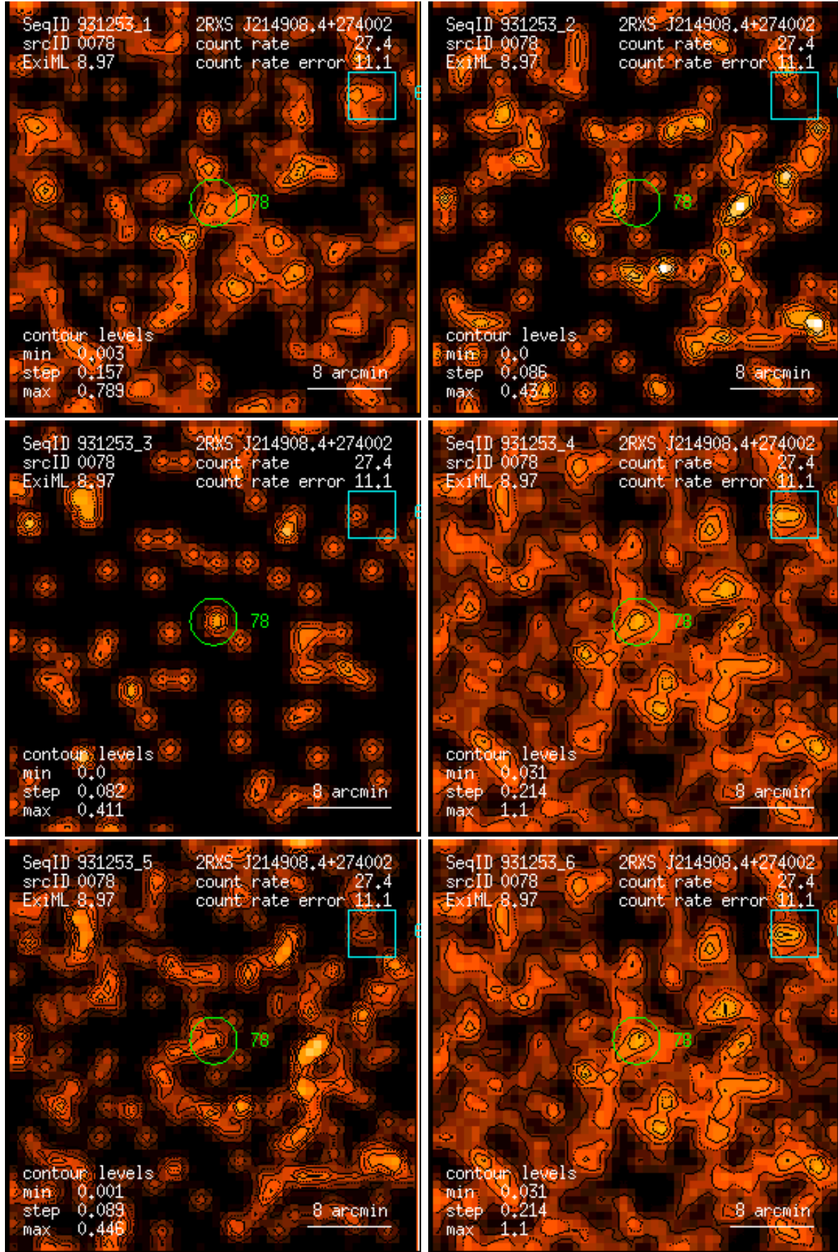
Figure 78: RASS 931253: detection 0078: band rate images, Gaussian filter: (1) PSPC channels 11 – 41, (2) 52 – 90, (3) 91 – 201, (4) 11 – 235, (5) 52 – 201, (6) 11 – 201. Broad band rates in counts/ks. Band rate contour levels in counts/ks/arcmin 2 .
