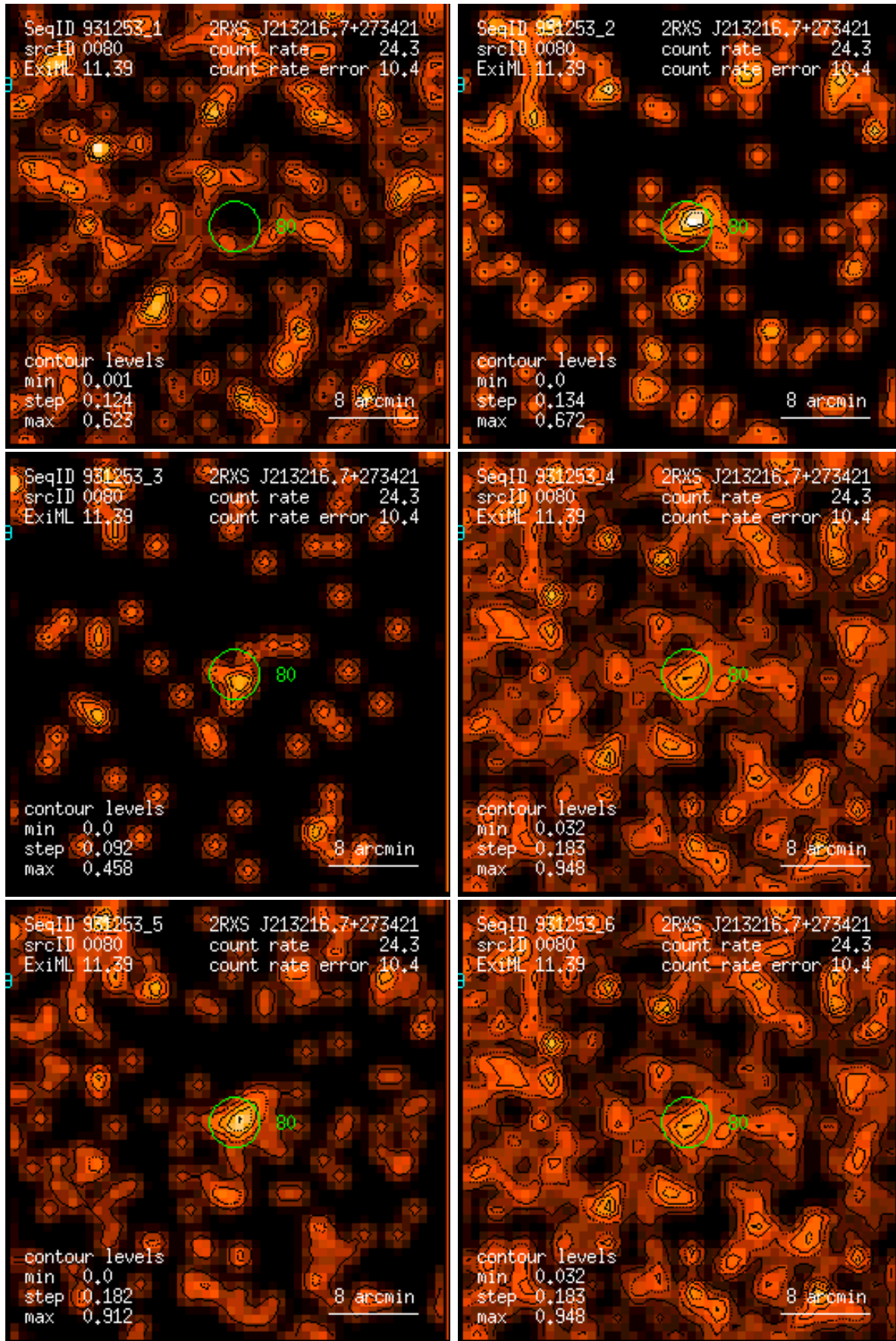
Figure 80: RASS 931253: detection 0080: band rate images, Gaussian filter: (1) PSPC channels 11 – 41, (2) 52 – 90, (3) 91 – 201, (4) 11 – 235, (5) 52 – 201, (6) 11 – 201. Broad band rates in counts/ks. Band rate contour levels in counts/ks/arcmin 2 .
