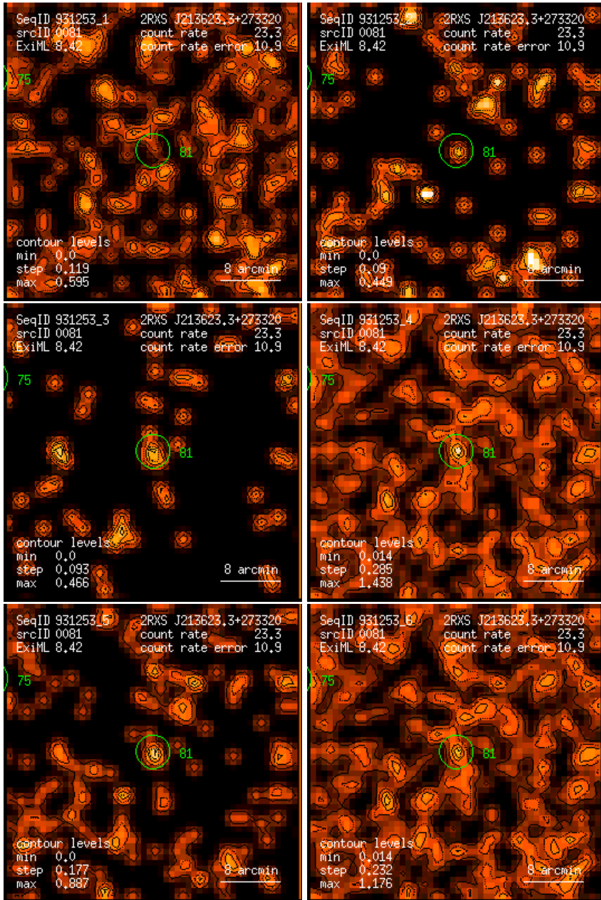
Figure 81: RASS 931253: detection 0081: band rate images, Gaussian filter: (1) PSPC channels 11 – 41, (2) 52 – 90, (3) 91 – 201, (4) 11 – 235, (5) 52 – 201, (6) 11 – 201. Broad band rates in counts/ks. Band rate contour levels in counts/ks/arcmin 2 .
