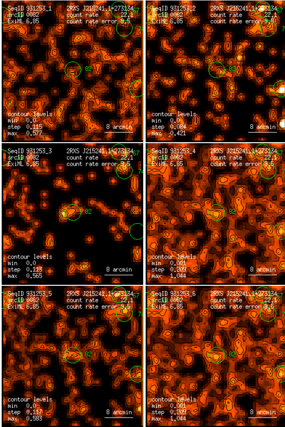
Figure 82: RASS 931253: detection 0082: band rate images, Gaussian filter: (1) PSPC channels 11 – 41, (2) 52 – 90, (3) 91 – 201, (4) 11 – 235, (5) 52 – 201, (6) 11 – 201. Broad band rates in counts/ks. Band rate contour levels in counts/ks/arcmin 2 .
