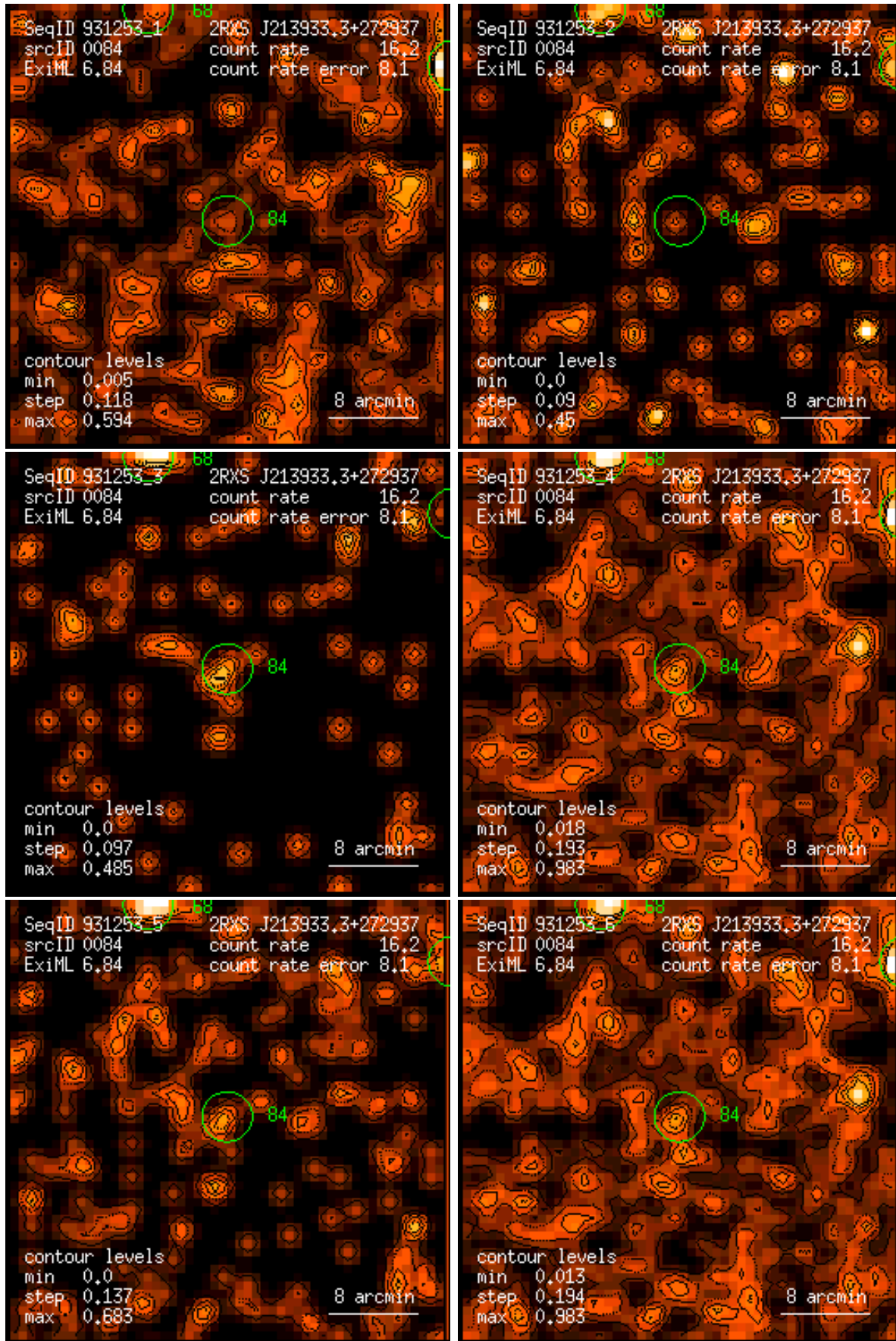
Figure 84: RASS 931253: detection 0084: band rate images, Gaussian filter: (1) PSPC channels 11 – 41, (2) 52 – 90, (3) 91 – 201, (4) 11 – 235, (5) 52 – 201, (6) 11 – 201. Broad band rates in counts/ks. Band rate contour levels in counts/ks/arcmin 2 .
