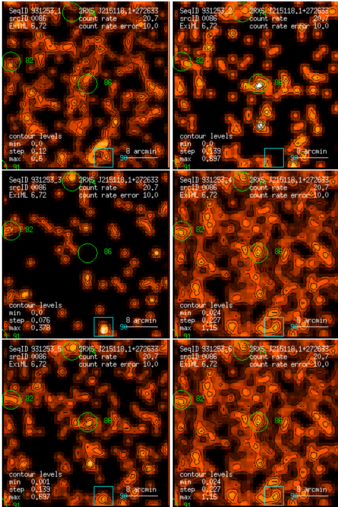
Figure 86: RASS 931253: detection 0086: band rate images, Gaussian filter: (1) PSPC channels 11 – 41, (2) 52 – 90, (3) 91 – 201, (4) 11 – 235, (5) 52 – 201, (6) 11 – 201. Broad band rates in counts/ks. Band rate contour levels in counts/ks/arcmin 2 .
