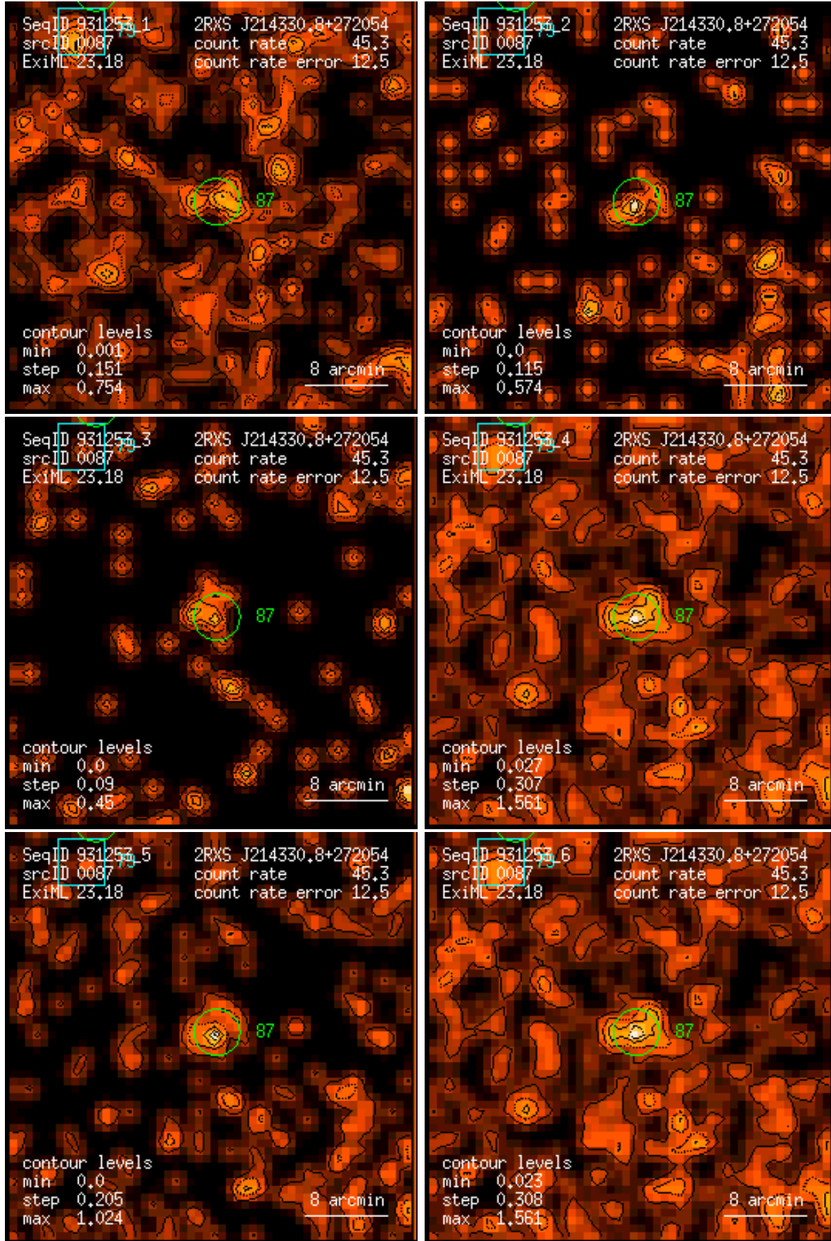
Figure 87: RASS 931253: detection 0087: band rate images, Gaussian filter: (1) PSPC channels 11 – 41, (2) 52 – 90, (3) 91 – 201, (4) 11 – 235, (5) 52 – 201, (6) 11 – 201. Broad band rates in counts/ks. Band rate contour levels in counts/ks/arcmin 2 .
