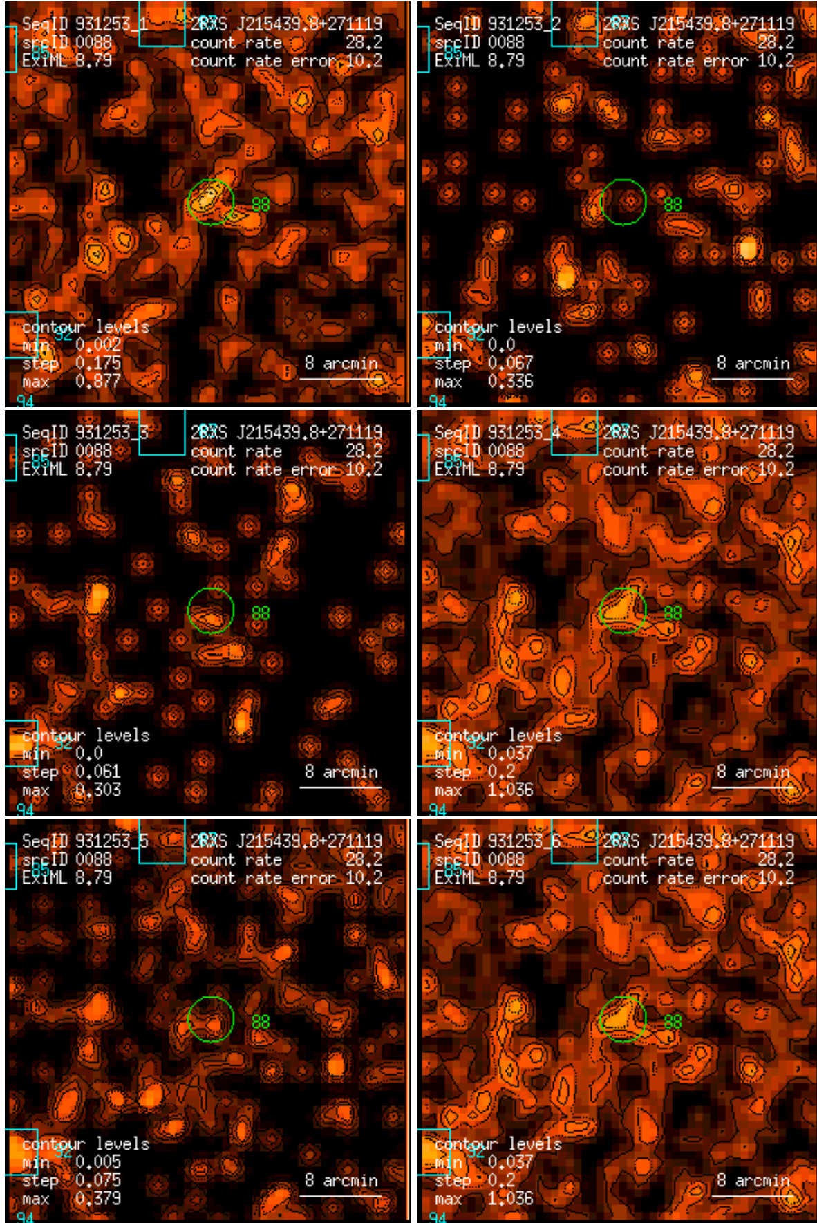
Figure 88: RASS 931253: detection 0088: band rate images, Gaussian filter: (1) PSPC channels 11 – 41, (2) 52 – 90, (3) 91 – 201, (4) 11 – 235, (5) 52 – 201, (6) 11 – 201. Broad band rates in counts/ks. Band rate contour levels in counts/ks/arcmin 2 .
