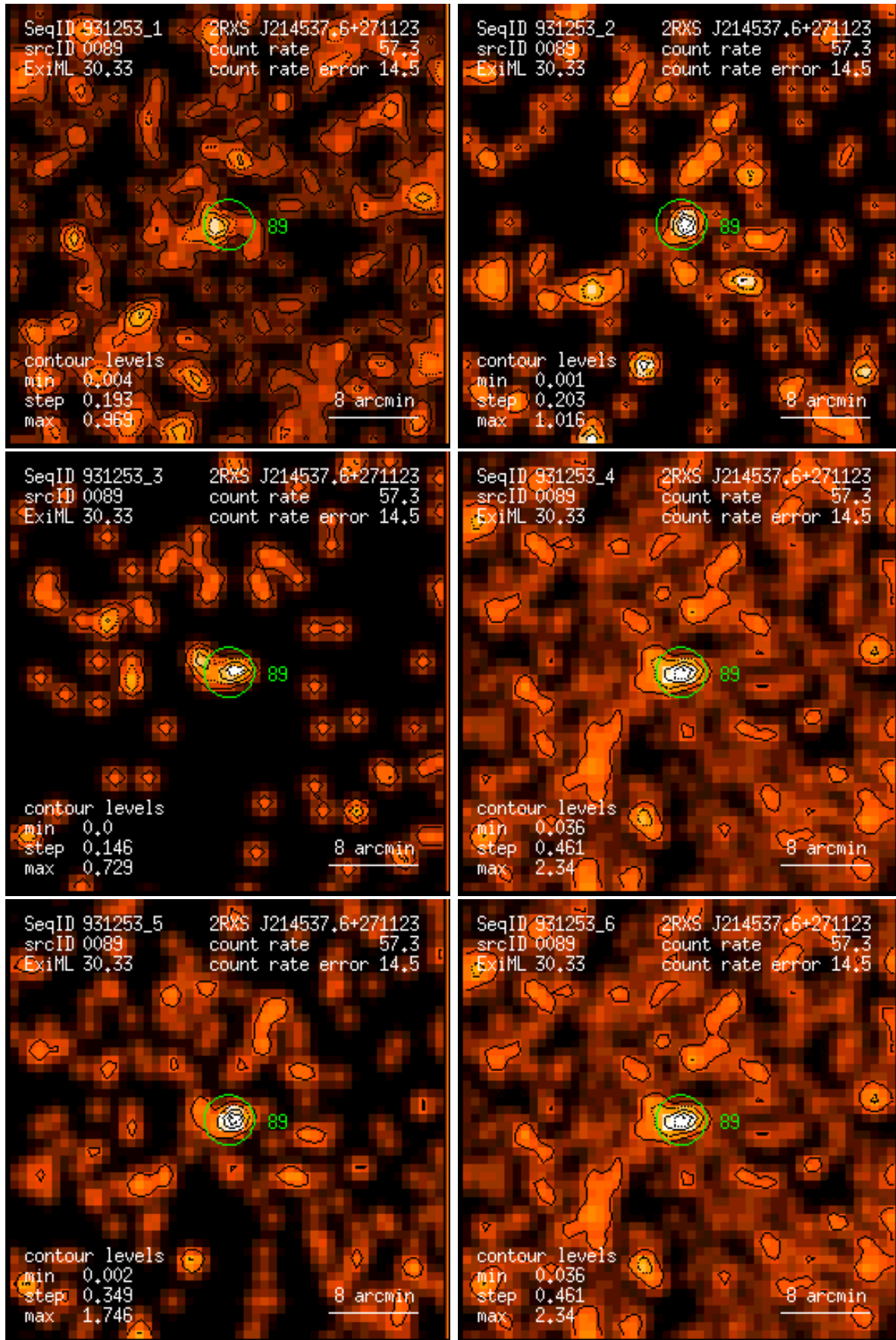
Figure 89: RASS 931253: detection 0089: band rate images, Gaussian filter: (1) PSPC channels 11 – 41, (2) 52 – 90, (3) 91 – 201, (4) 11 – 235, (5) 52 – 201, (6) 11 – 201. Broad band rates in counts/ks. Band rate contour levels in counts/ks/arcmin 2 .
