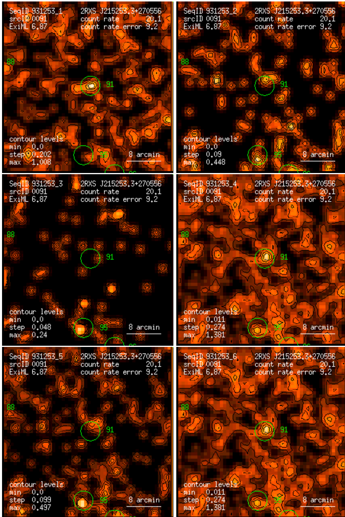
Figure 91: RASS 931253: detection 0091: band rate images, Gaussian filter: (1) PSPC channels 11 – 41, (2) 52 – 90, (3) 91 – 201, (4) 11 – 235, (5) 52 – 201, (6) 11 – 201. Broad band rates in counts/ks. Band rate contour levels in counts/ks/arcmin 2 .
