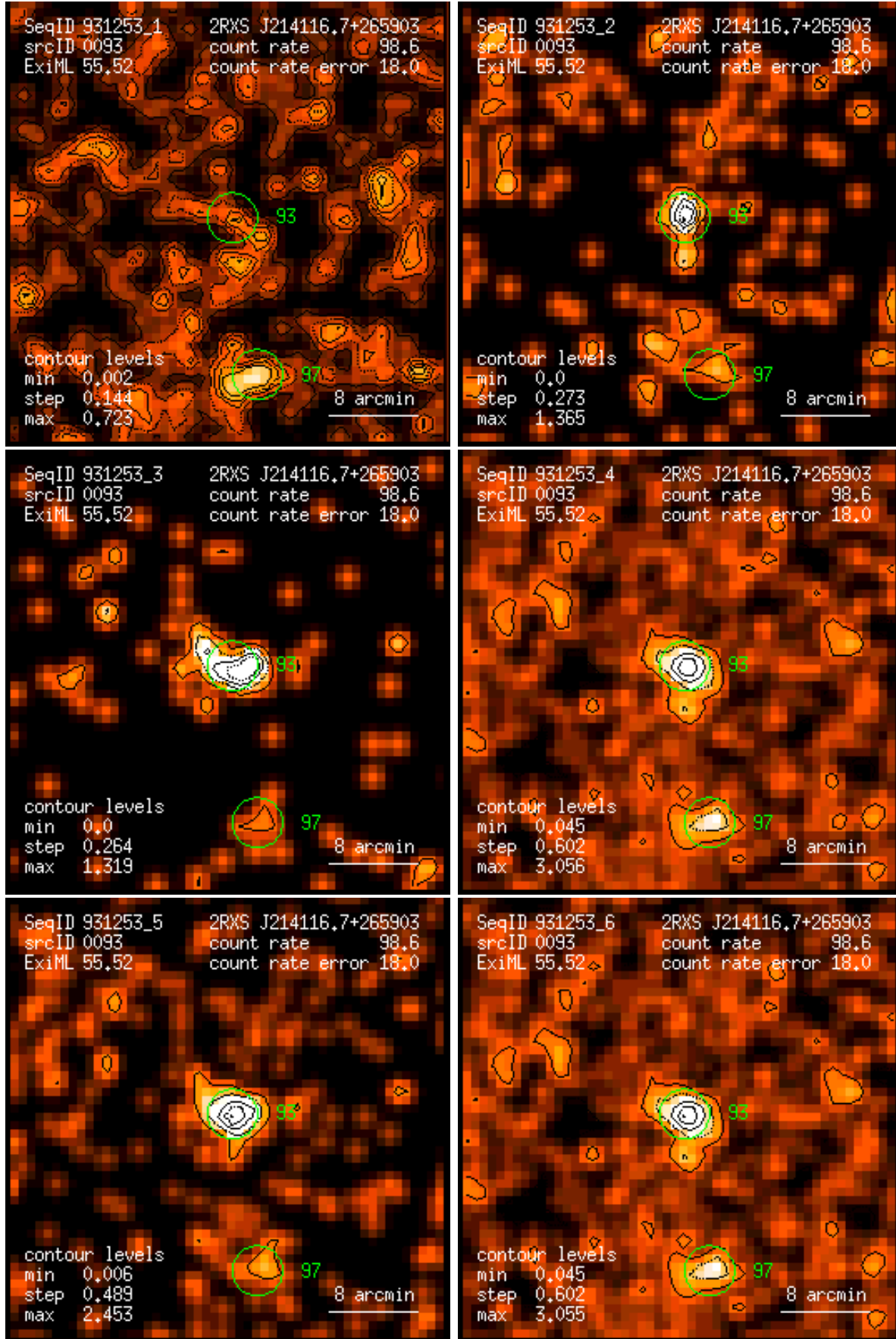
Figure 93: RASS 931253: detection 0093: band rate images, Gaussian filter: (1) PSPC channels 11 – 41, (2) 52 – 90, (3) 91 – 201, (4) 11 – 235, (5) 52 – 201, (6) 11 – 201. Broad band rates in counts/ks. Band rate contour levels in counts/ks/arcmin 2 .
