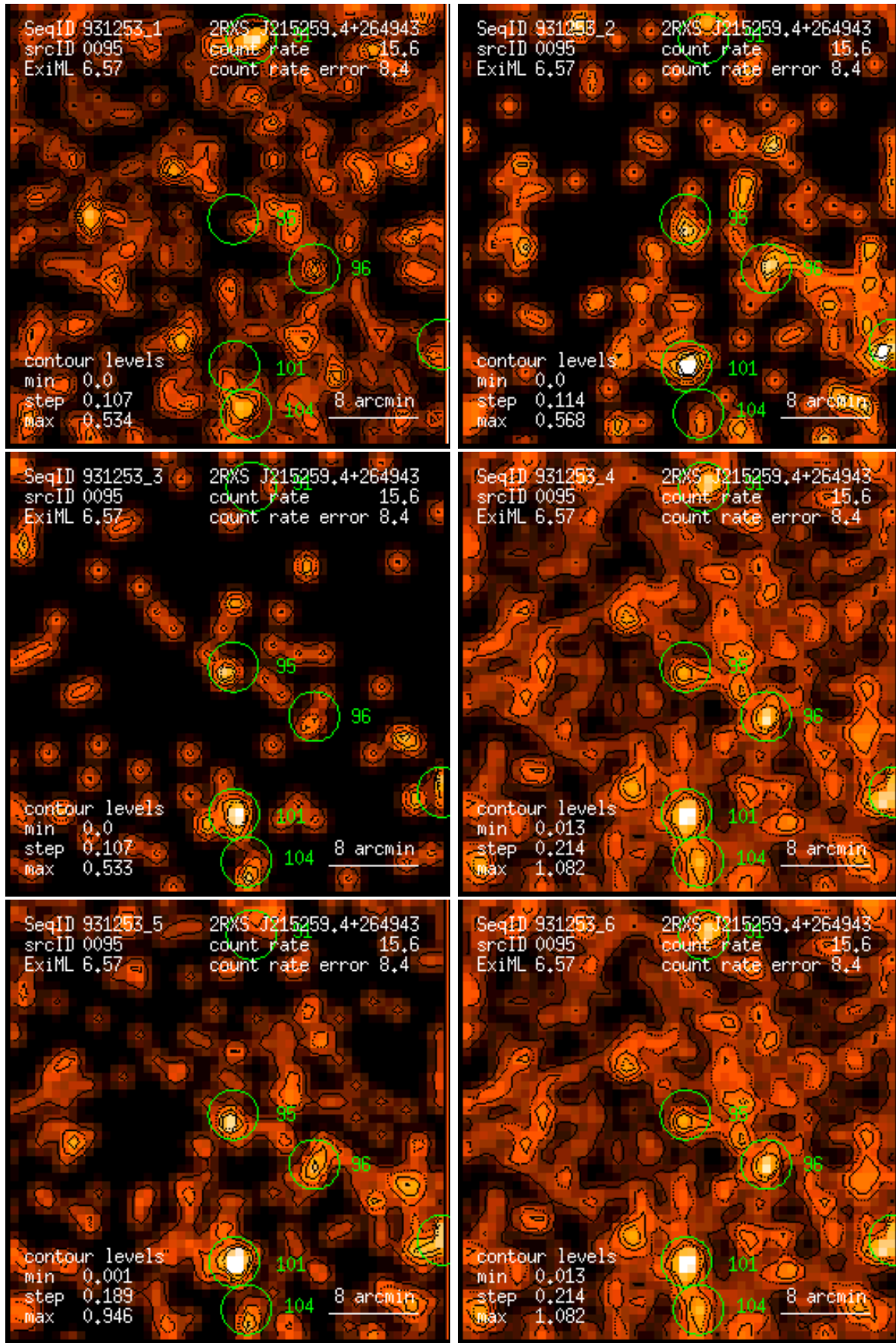
Figure 95: RASS 931253: detection 0095: band rate images, Gaussian filter: (1) PSPC channels 11 – 41, (2) 52 – 90, (3) 91 – 201, (4) 11 – 235, (5) 52 – 201, (6) 11 – 201. Broad band rates in counts/ks. Band rate contour levels in counts/ks/arcmin 2 .
