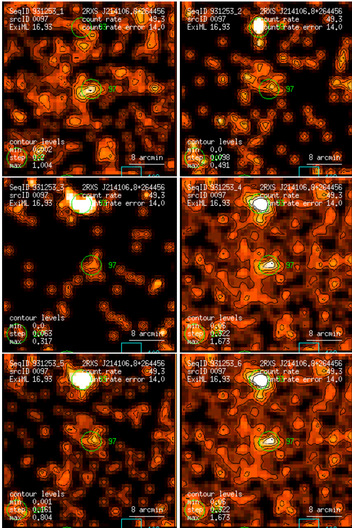
Figure 97: RASS 931253: detection 0097: band rate images, Gaussian filter: (1) PSPC channels 11 – 41, (2) 52 – 90, (3) 91 – 201, (4) 11 – 235, (5) 52 – 201, (6) 11 – 201. Broad band rates in counts/ks. Band rate contour levels in counts/ks/arcmin 2 .
