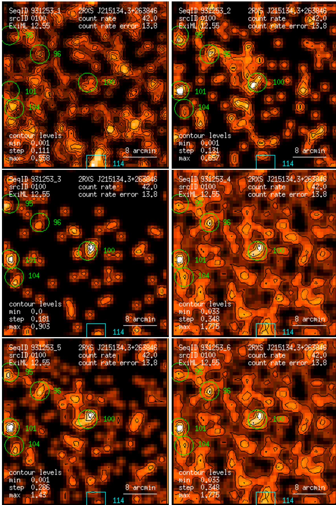
Figure 100: RASS 931253: detection 0100: band rate images, Gaussian filter: (1) PSPC channels 11 – 41, (2) 52 – 90, (3) 91 – 201, (4) 11 – 235, (5) 52 – 201, (6) 11 – 201. Broad band rates in counts/ks. Band rate contour levels in counts/ks/arcmin 2 .
