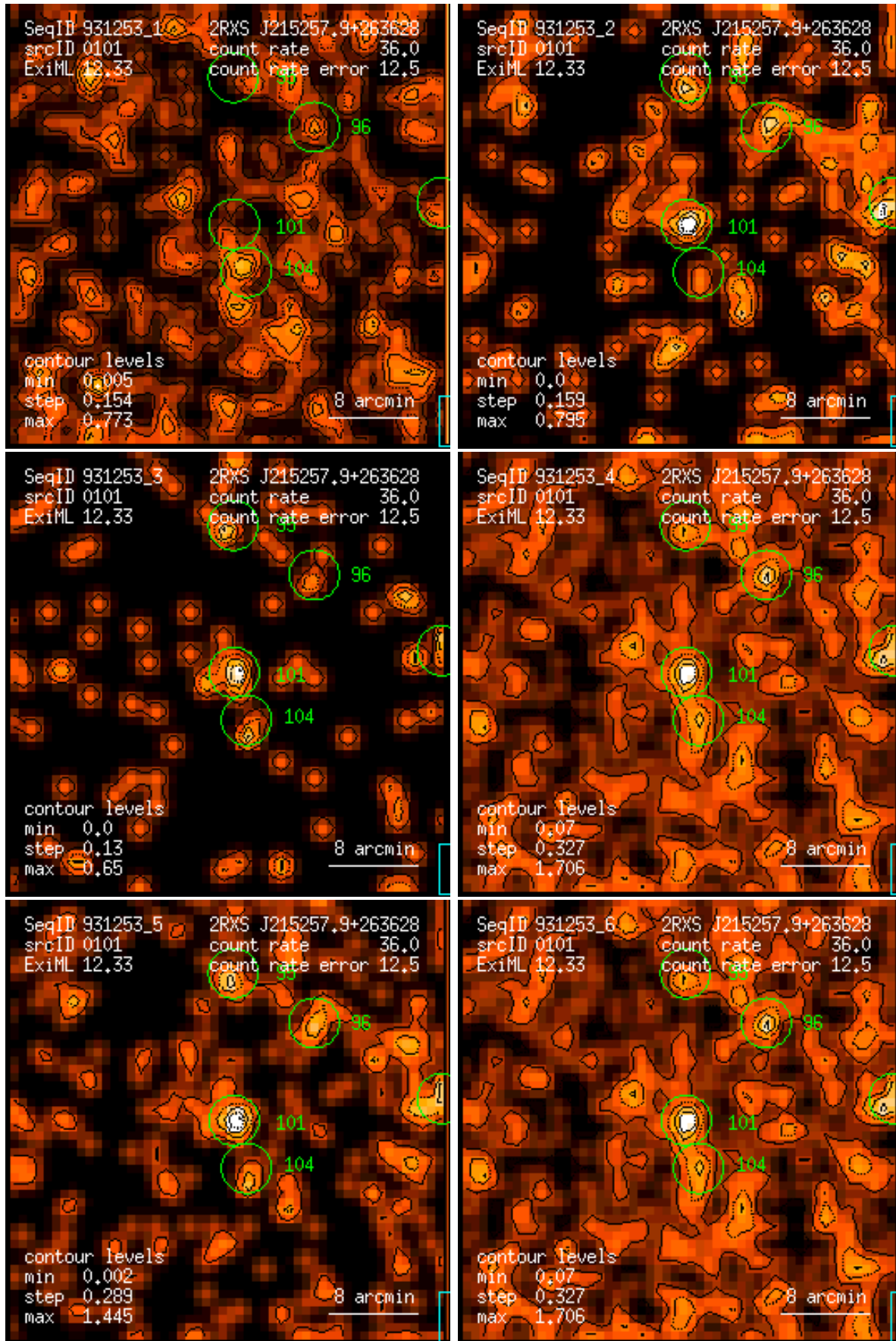
Figure 101: RASS 931253: detection 0101: band rate images, Gaussian filter: (1) PSPC channels 11 – 41, (2) 52 – 90, (3) 91 – 201, (4) 11 – 235, (5) 52 – 201, (6) 11 – 201. Broad band rates in counts/ks. Band rate contour levels in counts/ks/arcmin 2 .
