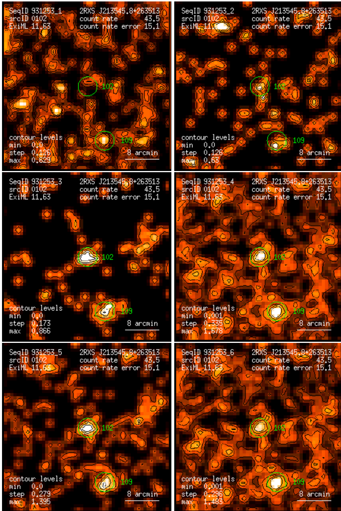
Figure 102: RASS 931253: detection 0102: band rate images, Gaussian filter: (1) PSPC channels 11 – 41, (2) 52 – 90, (3) 91 – 201, (4) 11 – 235, (5) 52 – 201, (6) 11 – 201. Broad band rates in counts/ks. Band rate contour levels in counts/ks/arcmin 2 .
