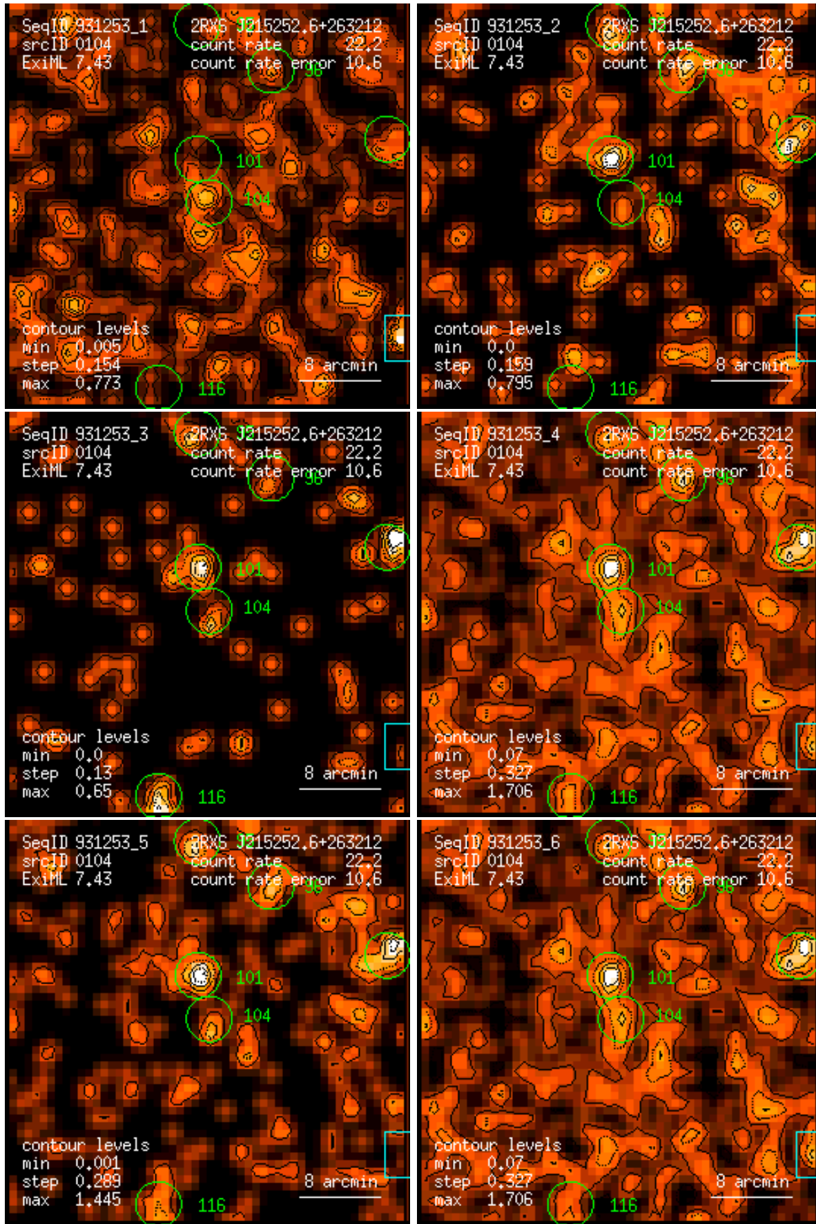
Figure 104: RASS 931253: detection 0104: band rate images, Gaussian filter: (1) PSPC channels 11 – 41, (2) 52 – 90, (3) 91 – 201, (4) 11 – 235, (5) 52 – 201, (6) 11 – 201. Broad band rates in counts/ks. Band rate contour levels in counts/ks/arcmin 2 .
