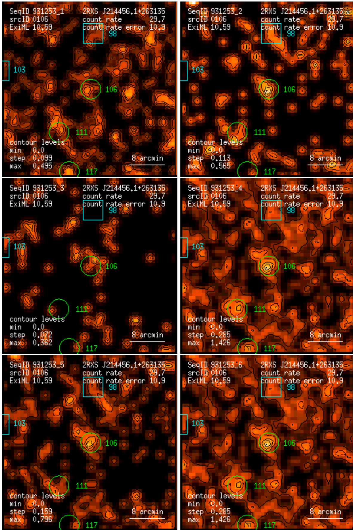
Figure 106: RASS 931253: detection 0106: band rate images, Gaussian filter: (1) PSPC channels 11 – 41, (2) 52 – 90, (3) 91 – 201, (4) 11 – 235, (5) 52 – 201, (6) 11 – 201. Broad band rates in counts/ks. Band rate contour levels in counts/ks/arcmin 2 .
