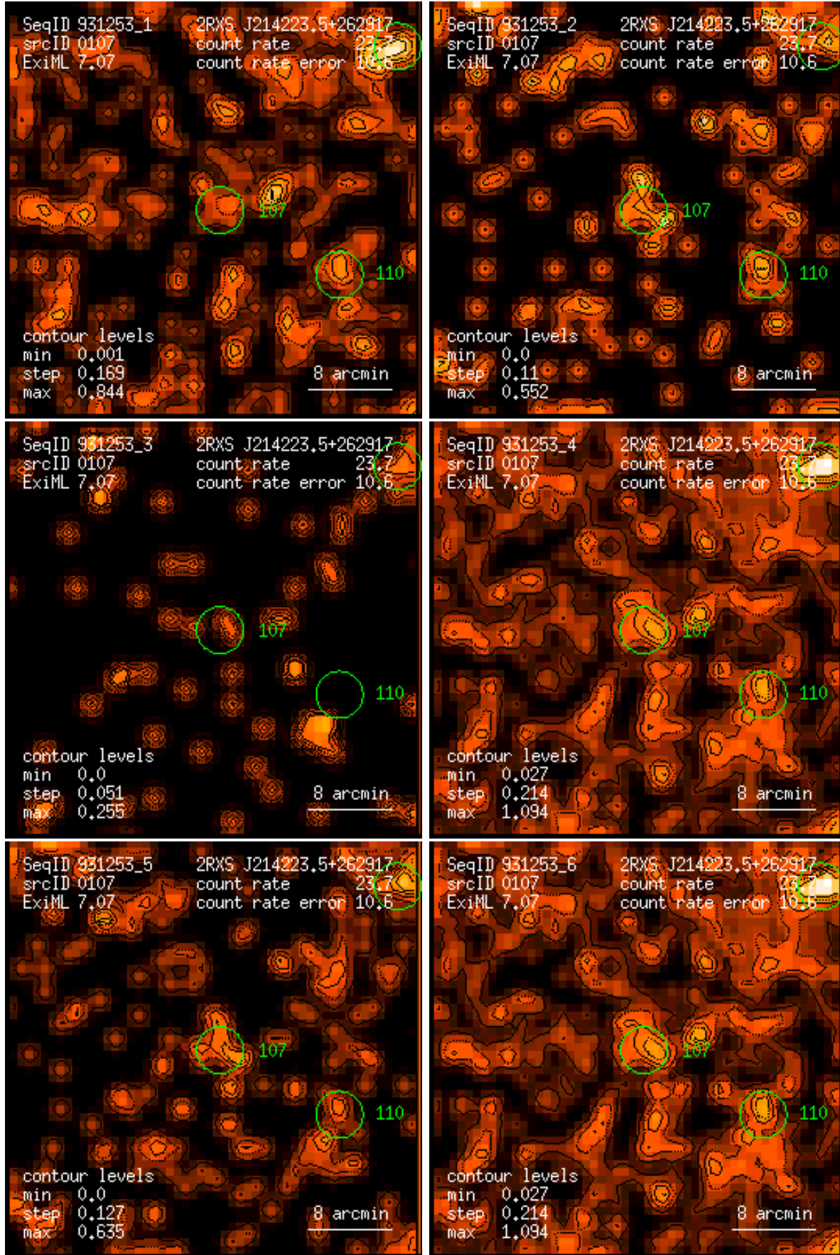
Figure 107: RASS 931253: detection 0107: band rate images, Gaussian filter: (1) PSPC channels 11 – 41, (2) 52 – 90, (3) 91 – 201, (4) 11 – 235, (5) 52 – 201, (6) 11 – 201. Broad band rates in counts/ks. Band rate contour levels in counts/ks/arcmin 2 .
