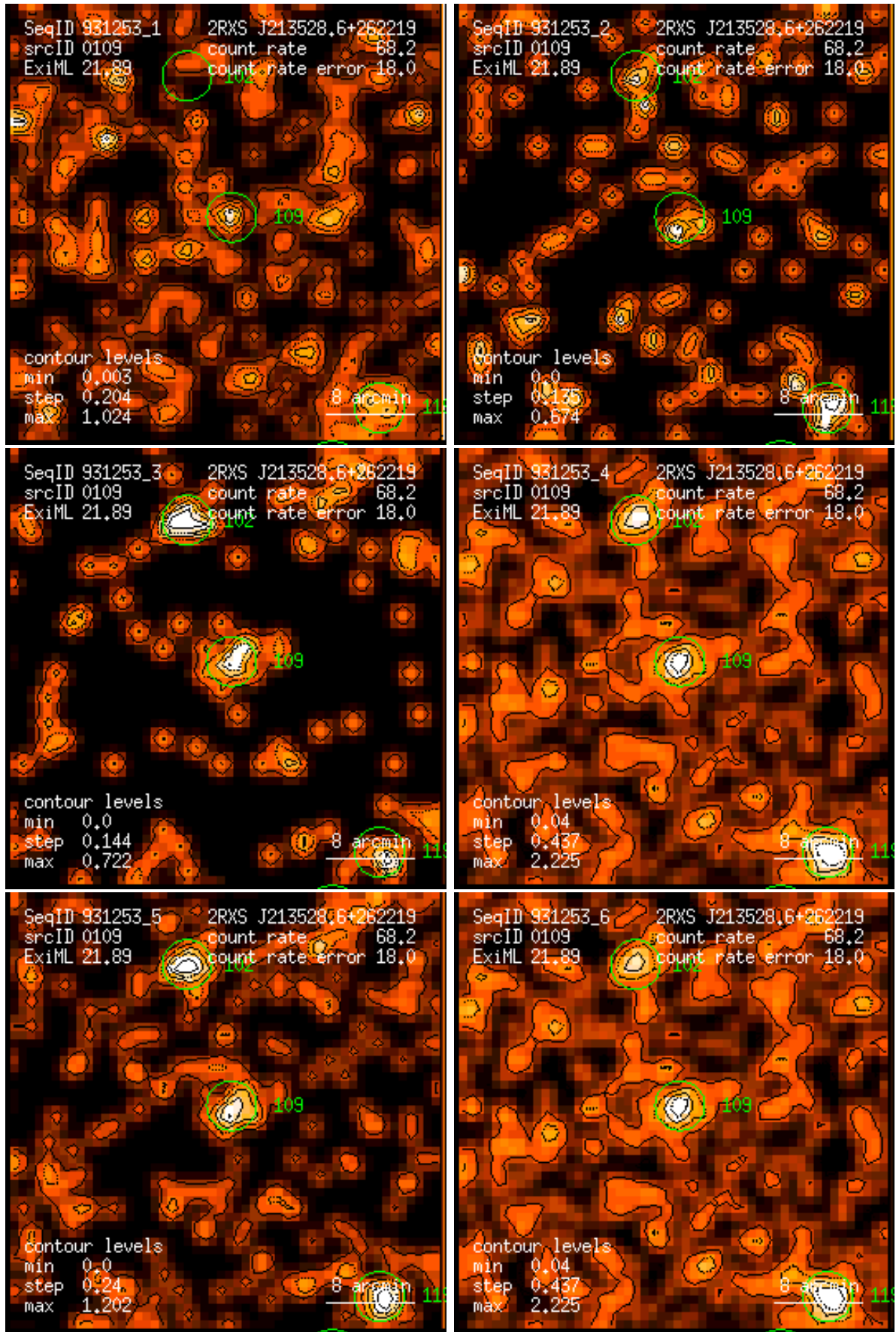
Figure 109: RASS 931253: detection 0109: band rate images, Gaussian filter: (1) PSPC channels 11 – 41, (2) 52 – 90, (3) 91 – 201, (4) 11 – 235, (5) 52 – 201, (6) 11 – 201. Broad band rates in counts/ks. Band rate contour levels in counts/ks/arcmin 2 .
