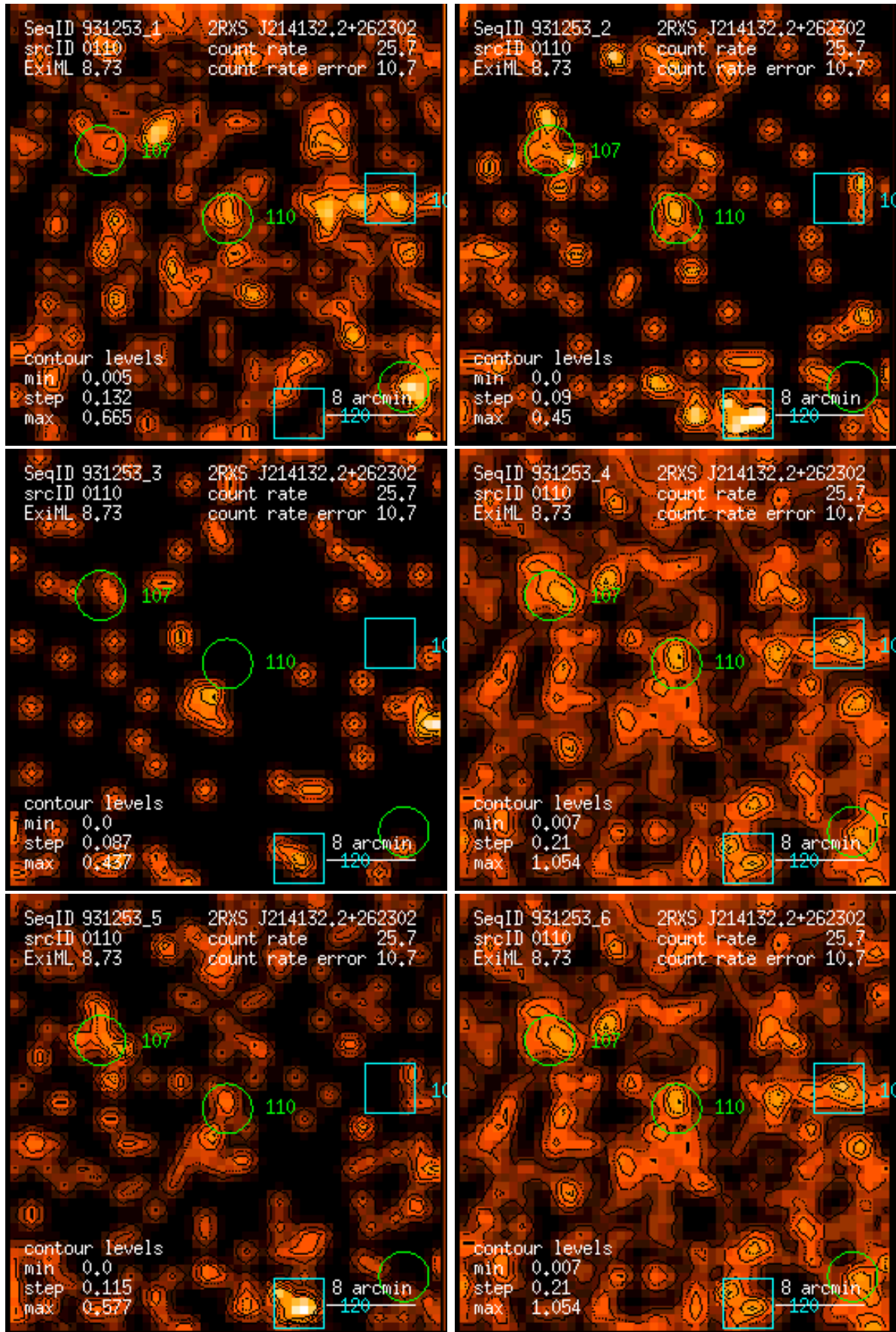
Figure 110: RASS 931253: detection 0110: band rate images, Gaussian filter: (1) PSPC channels 11 – 41, (2) 52 – 90, (3) 91 – 201, (4) 11 – 235, (5) 52 – 201, (6) 11 – 201. Broad band rates in counts/ks. Band rate contour levels in counts/ks/arcmin 2 .
