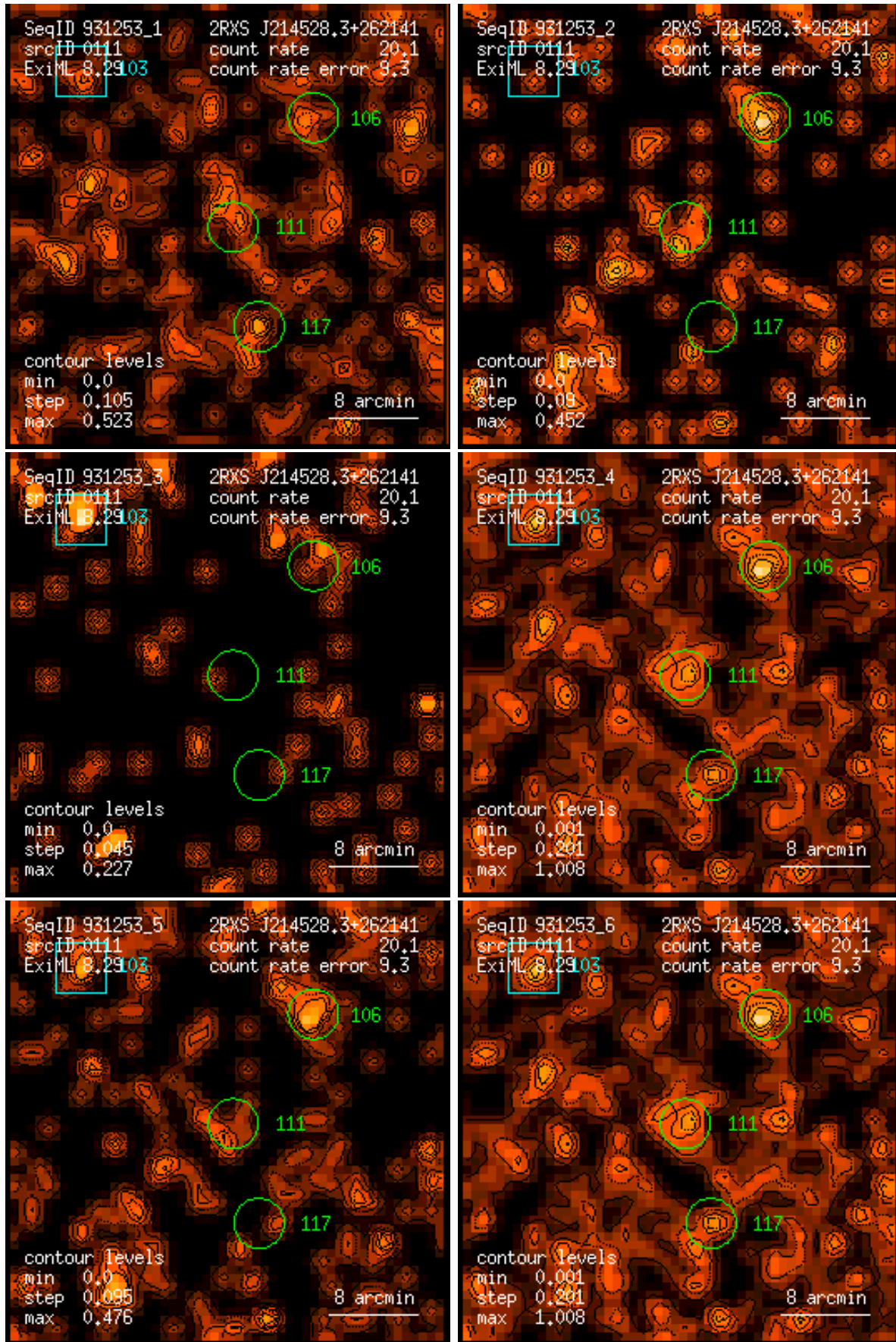
Figure 111: RASS 931253: detection 0111: band rate images, Gaussian filter: (1) PSPC channels 11 – 41, (2) 52 – 90, (3) 91 – 201, (4) 11 – 235, (5) 52 – 201, (6) 11 – 201. Broad band rates in counts/ks. Band rate contour levels in counts/ks/arcmin 2 .
