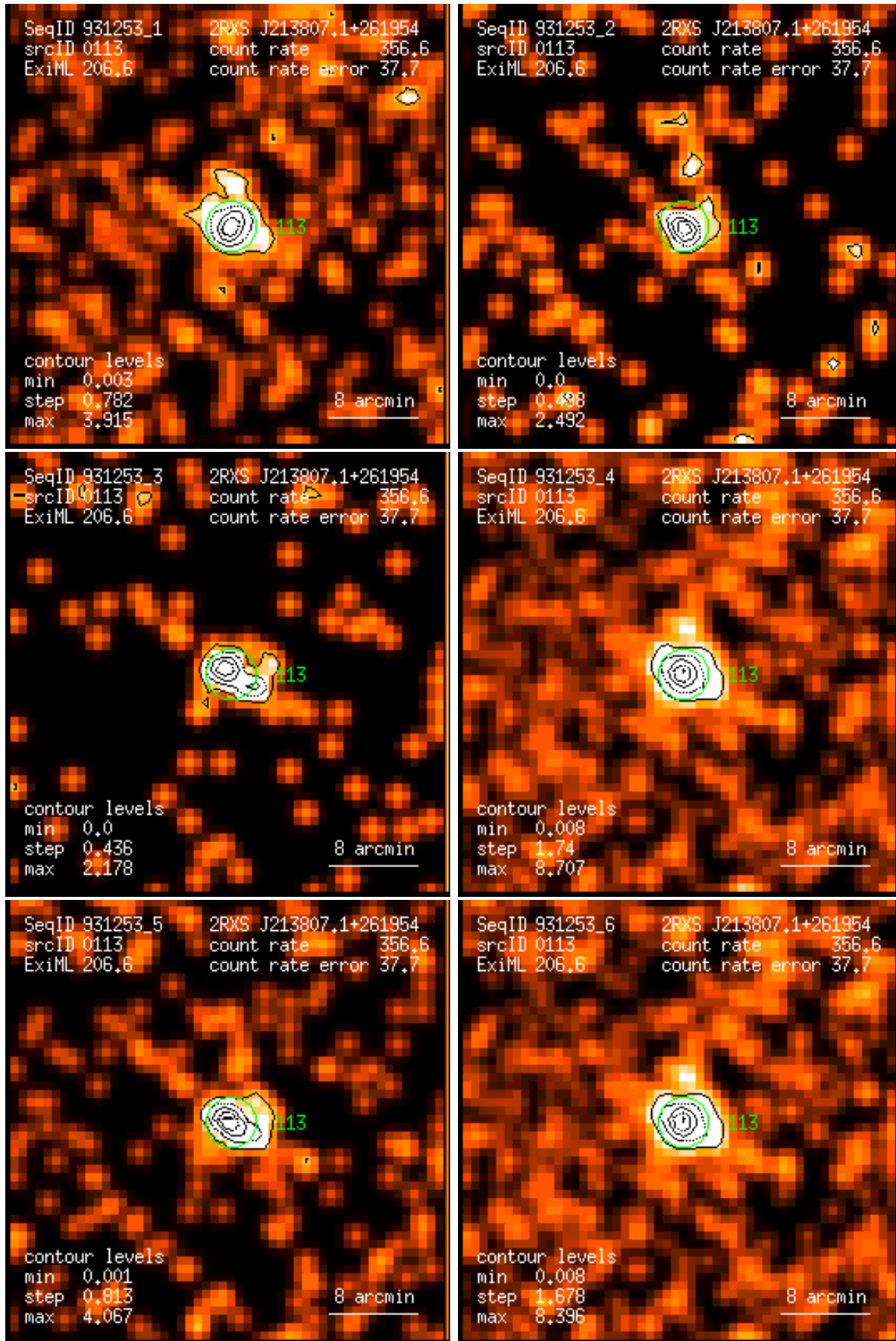
Figure 113: RASS 931253: detection 0113: band rate images, Gaussian filter: (1) PSPC channels 11 – 41, (2) 52 – 90, (3) 91 – 201, (4) 11 – 235, (5) 52 – 201, (6) 11 – 201. Broad band rates in counts/ks. Band rate contour levels in counts/ks/arcmin 2 .
