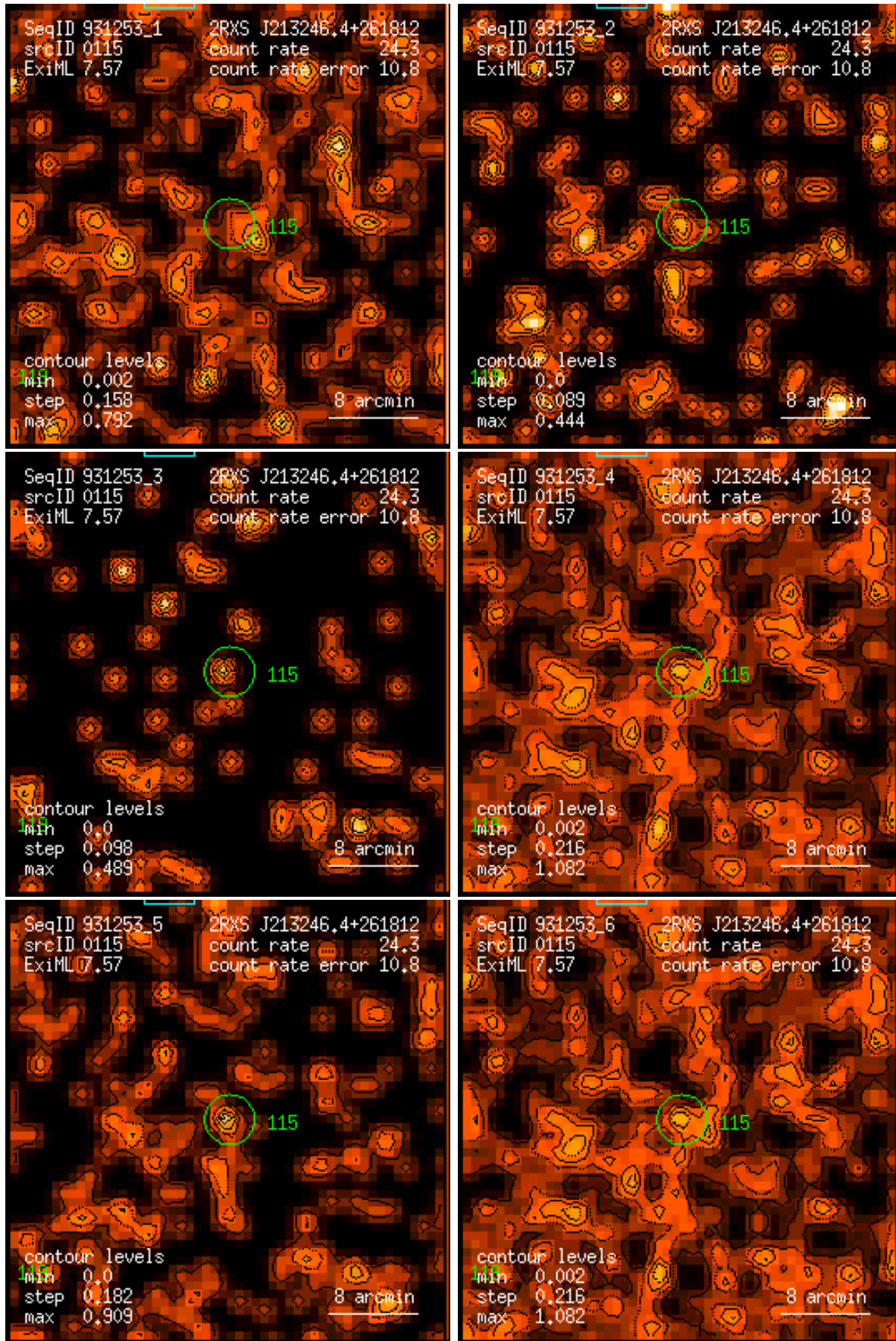
Figure 115: RASS 931253: detection 0115: band rate images, Gaussian filter: (1) PSPC channels 11 – 41, (2) 52 – 90, (3) 91 – 201, (4) 11 – 235, (5) 52 – 201, (6) 11 – 201. Broad band rates in counts/ks. Band rate contour levels in counts/ks/arcmin 2 .
