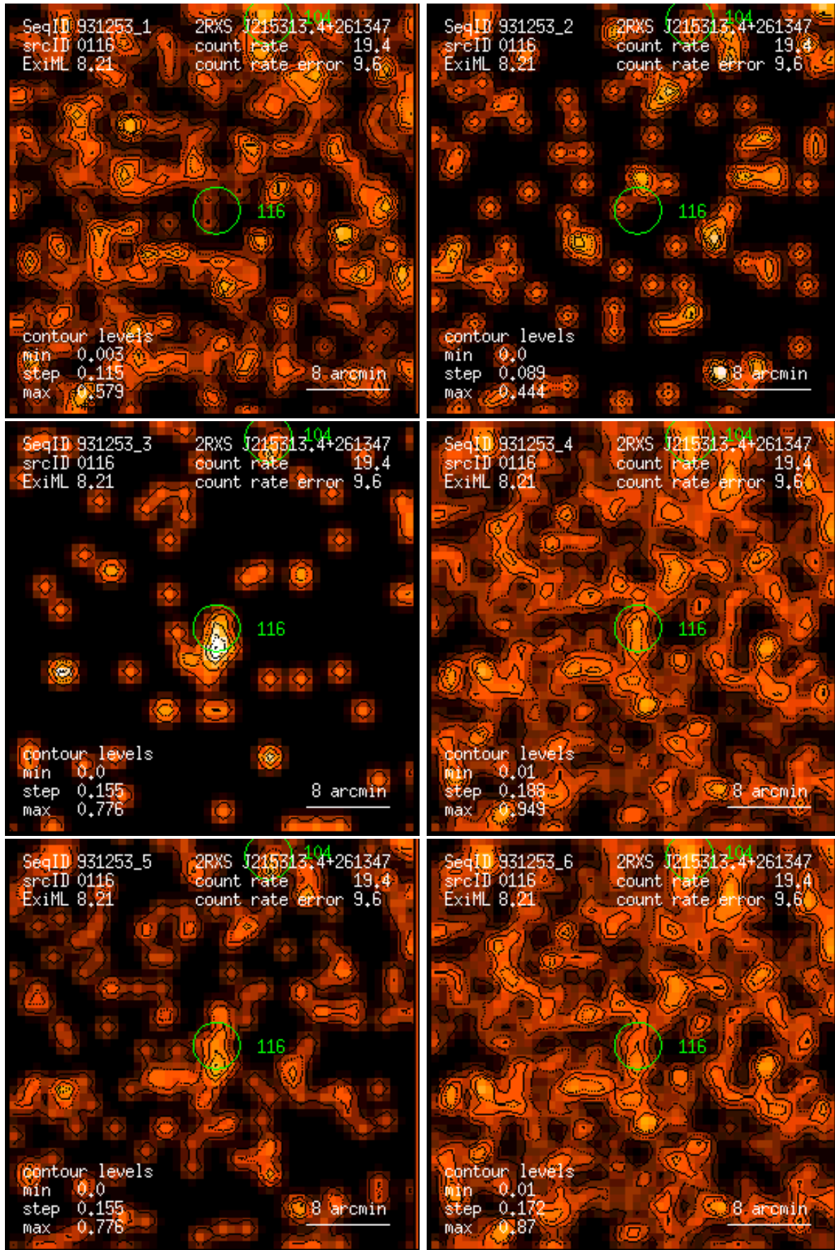
Figure 116: RASS 931253: detection 0116: band rate images, Gaussian filter: (1) PSPC channels 11 – 41, (2) 52 – 90, (3) 91 – 201, (4) 11 – 235, (5) 52 – 201, (6) 11 – 201. Broad band rates in counts/ks. Band rate contour levels in counts/ks/arcmin 2 .
