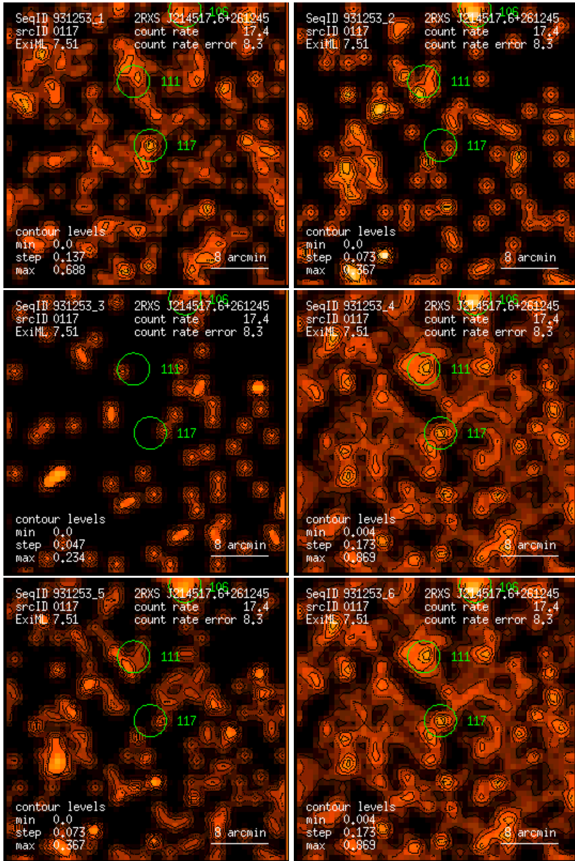
Figure 117: RASS 931253: detection 0117: band rate images, Gaussian filter: (1) PSPC channels 11 – 41, (2) 52 – 90, (3) 91 – 201, (4) 11 – 235, (5) 52 – 201, (6) 11 – 201. Broad band rates in counts/ks. Band rate contour levels in counts/ks/arcmin 2 .
