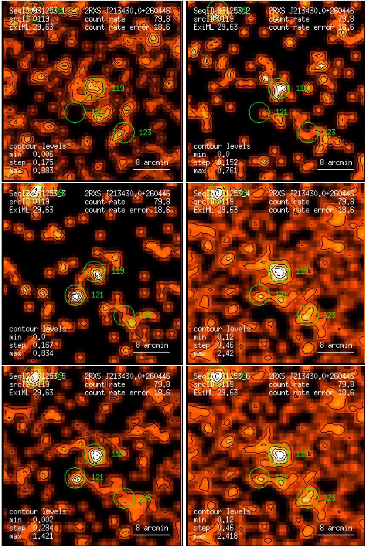
Figure 119: RASS 931253: detection 0119: band rate images, Gaussian filter: (1) PSPC channels 11 – 41, (2) 52 – 90, (3) 91 – 201, (4) 11 – 235, (5) 52 – 201, (6) 11 – 201. Broad band rates in counts/ks. Band rate contour levels in counts/ks/arcmin 2 .
