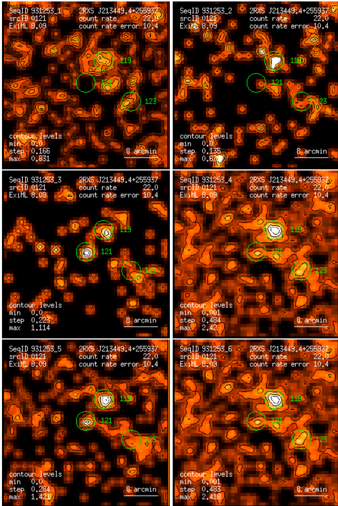
Figure 121: RASS 931253: detection 0121: band rate images, Gaussian filter: (1) PSPC channels 11 – 41, (2) 52 – 90, (3) 91 – 201, (4) 11 – 235, (5) 52 – 201, (6) 11 – 201. Broad band rates in counts/ks. Band rate contour levels in counts/ks/arcmin 2 .
