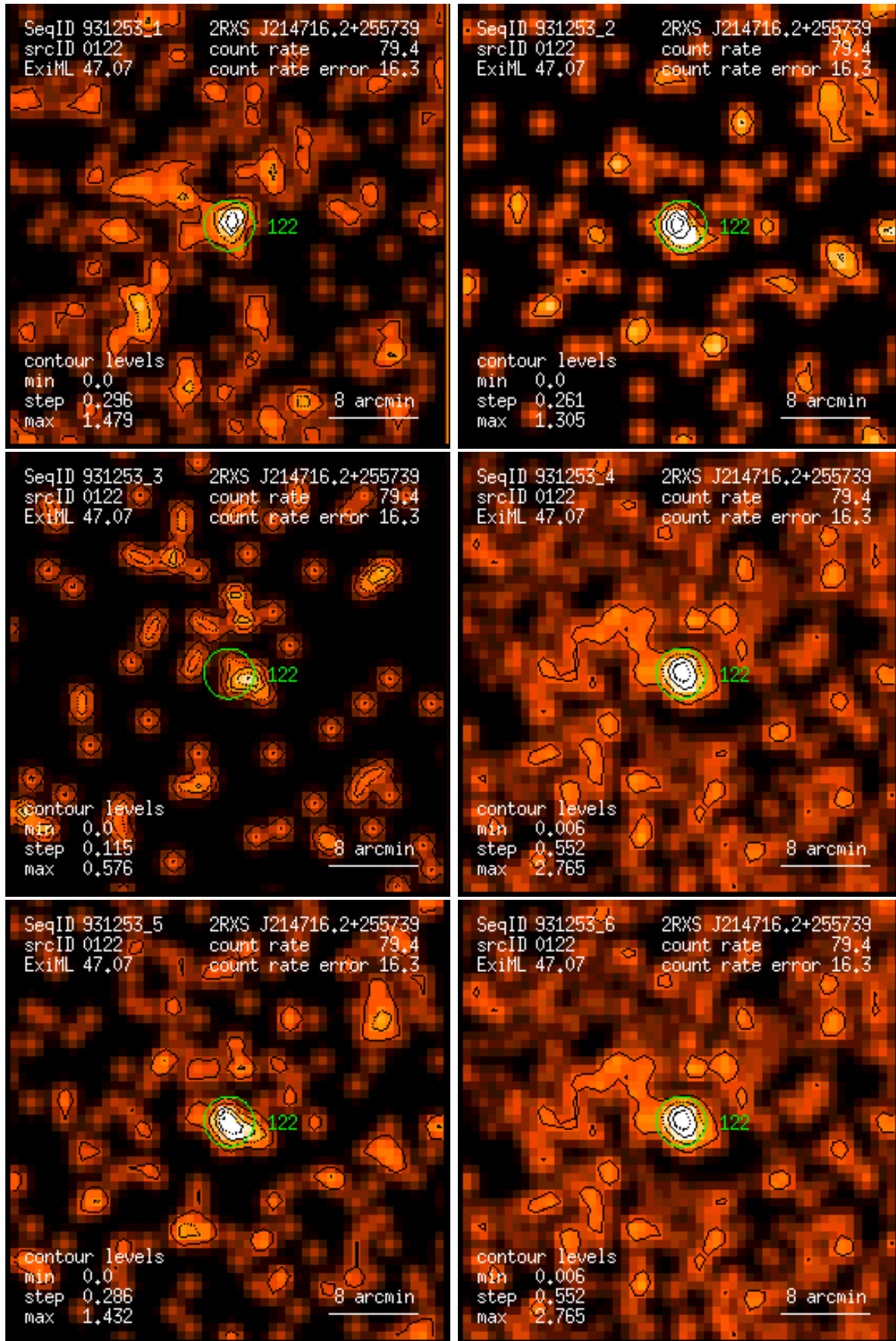
Figure 122: RASS 931253: detection 0122: band rate images, Gaussian filter: (1) PSPC channels 11 – 41, (2) 52 – 90, (3) 91 – 201, (4) 11 – 235, (5) 52 – 201, (6) 11 – 201. Broad band rates in counts/ks. Band rate contour levels in counts/ks/arcmin 2 .
