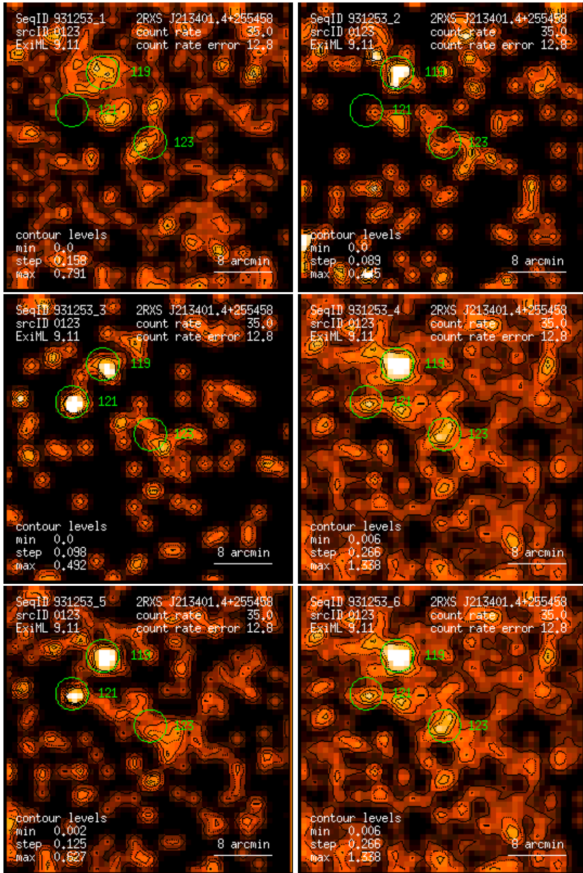
Figure 123: RASS 931253: detection 0123: band rate images, Gaussian filter: (1) PSPC channels 11 – 41, (2) 52 – 90, (3) 91 – 201, (4) 11 – 235, (5) 52 – 201, (6) 11 – 201. Broad band rates in counts/ks. Band rate contour levels in counts/ks/arcmin 2 .
