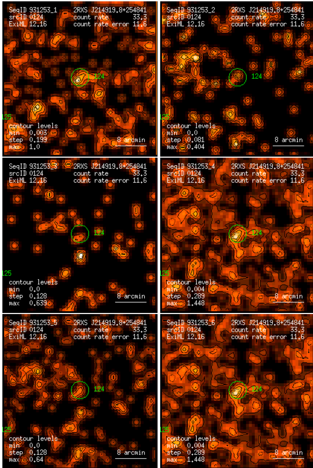
Figure 124: RASS 931253: detection 0124: band rate images, Gaussian filter: (1) PSPC channels 11 – 41, (2) 52 – 90, (3) 91 – 201, (4) 11 – 235, (5) 52 – 201, (6) 11 – 201. Broad band rates in counts/ks. Band rate contour levels in counts/ks/arcmin 2 .
