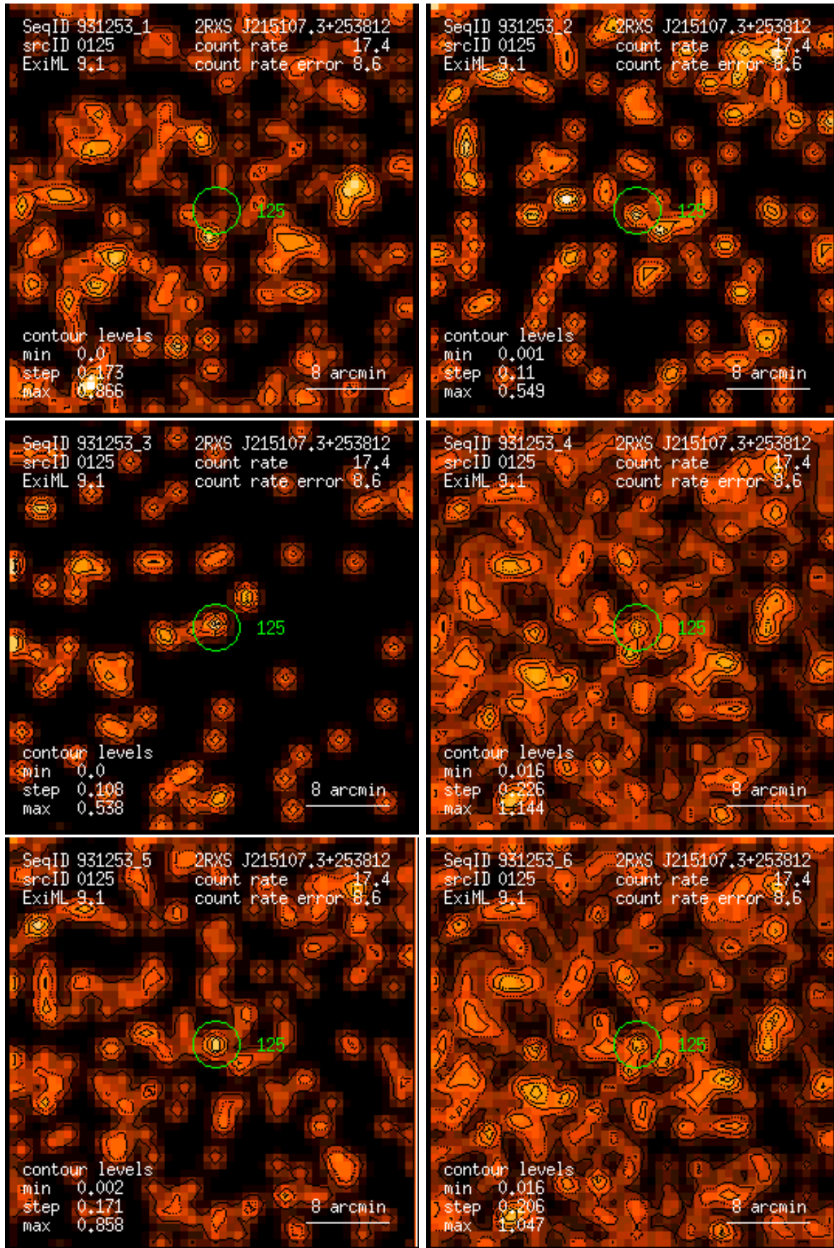
Figure 125: RASS 931253: detection 0125: band rate images, Gaussian filter: (1) PSPC channels 11 – 41, (2) 52 – 90, (3) 91 – 201, (4) 11 – 235, (5) 52 – 201, (6) 11 – 201. Broad band rates in counts/ks. Band rate contour levels in counts/ks/arcmin 2 .
