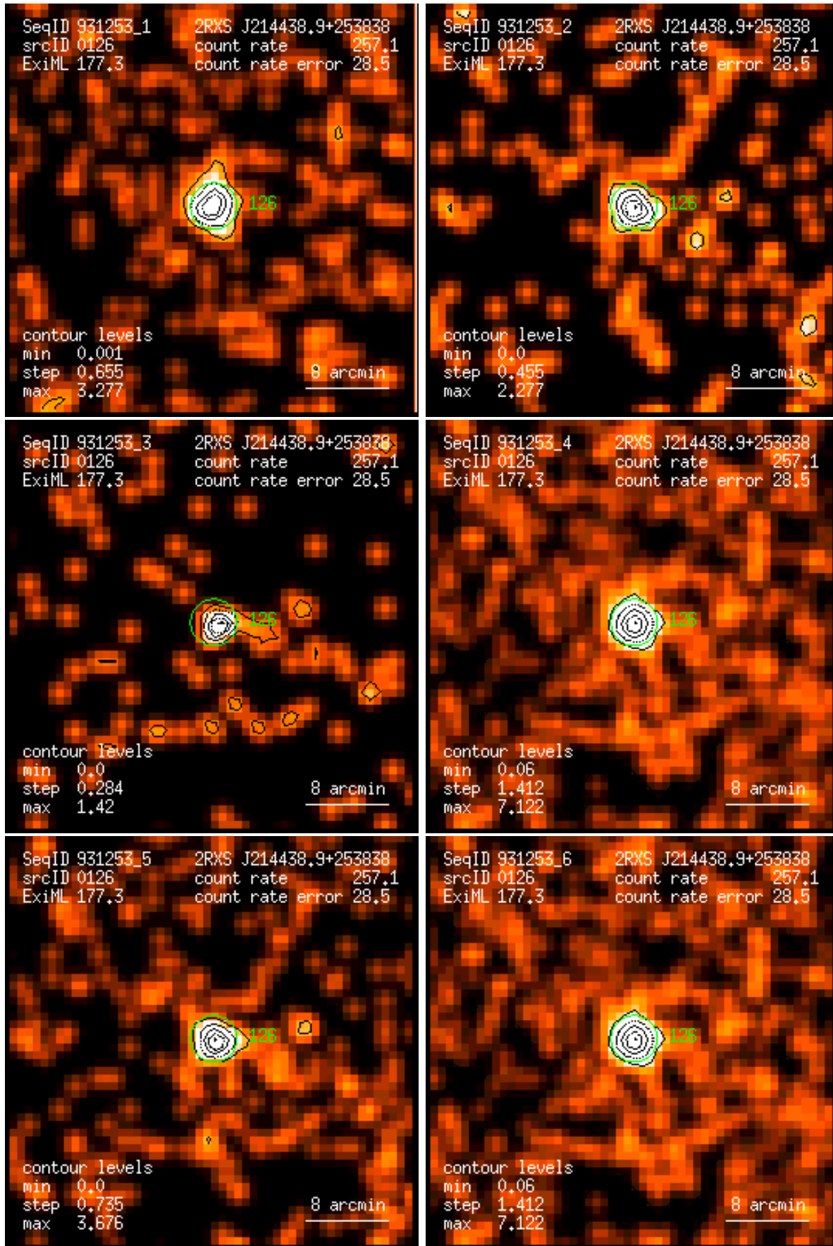
Figure 126: RASS 931253: detection 0126: band rate images, Gaussian filter: (1) PSPC channels 11 – 41, (2) 52 – 90, (3) 91 – 201, (4) 11 – 235, (5) 52 – 201, (6) 11 – 201. Broad band rates in counts/ks. Band rate contour levels in counts/ks/arcmin 2 .
