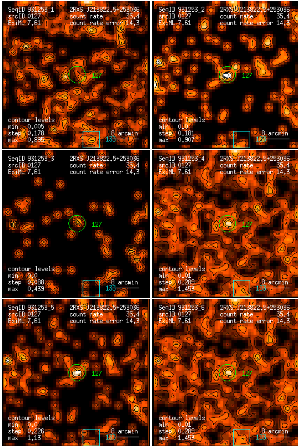
Figure 127: RASS 931253: detection 0127: band rate images, Gaussian filter: (1) PSPC channels 11 – 41, (2) 52 – 90, (3) 91 – 201, (4) 11 – 235, (5) 52 – 201, (6) 11 – 201. Broad band rates in counts/ks. Band rate contour levels in counts/ks/arcmin 2 .
