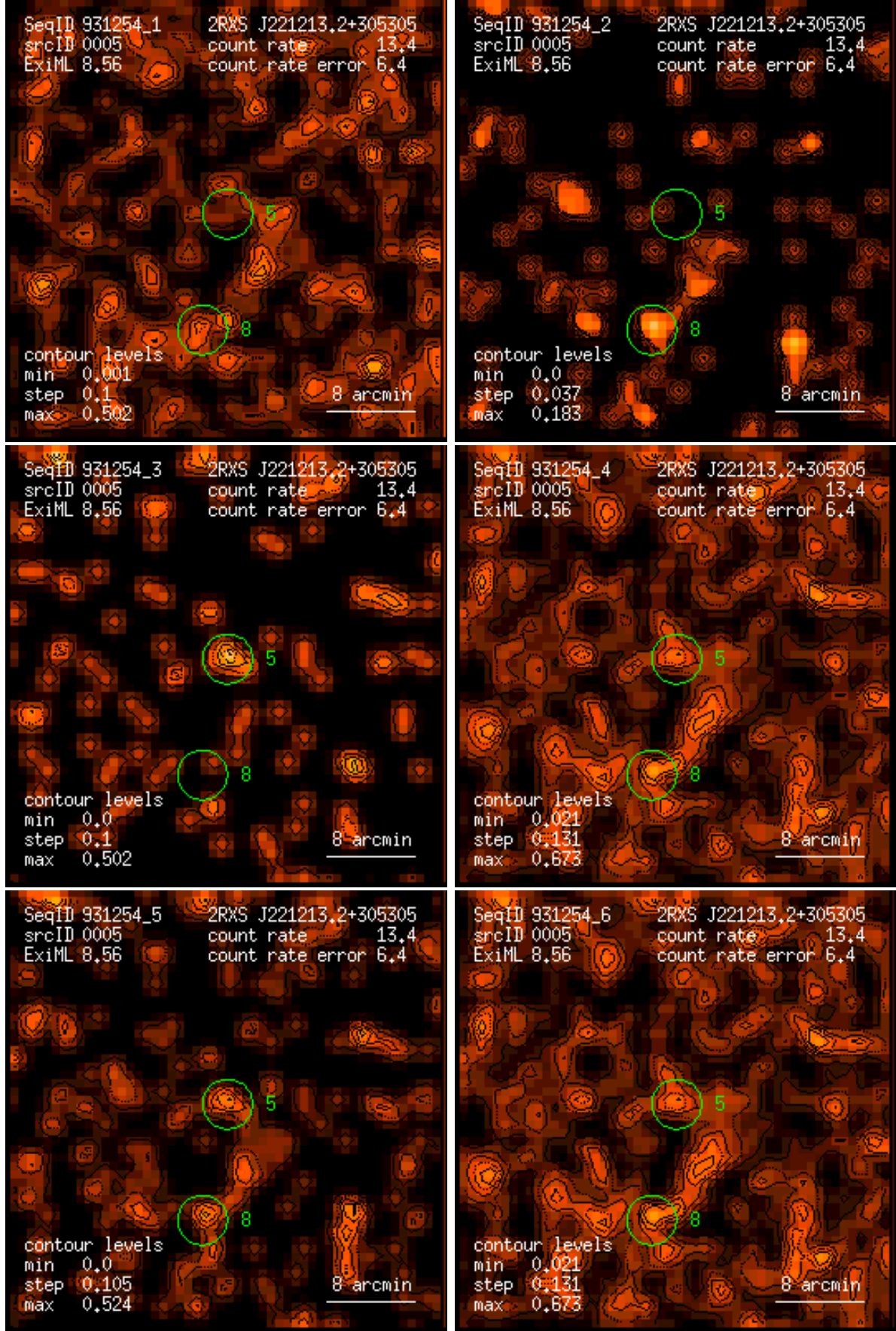
Figure 5: RASS 931254: detection 0005: band rate images, Gaussian filter: (1) PSPC channels 11 – 41, (2) 52 – 90, (3) 91 – 201, (4) 11 – 235, (5) 52 – 201, (6) 11 – 201. Broad band rates in counts/ks. Band rate contour levels in counts/ks/arcmin 2 .
