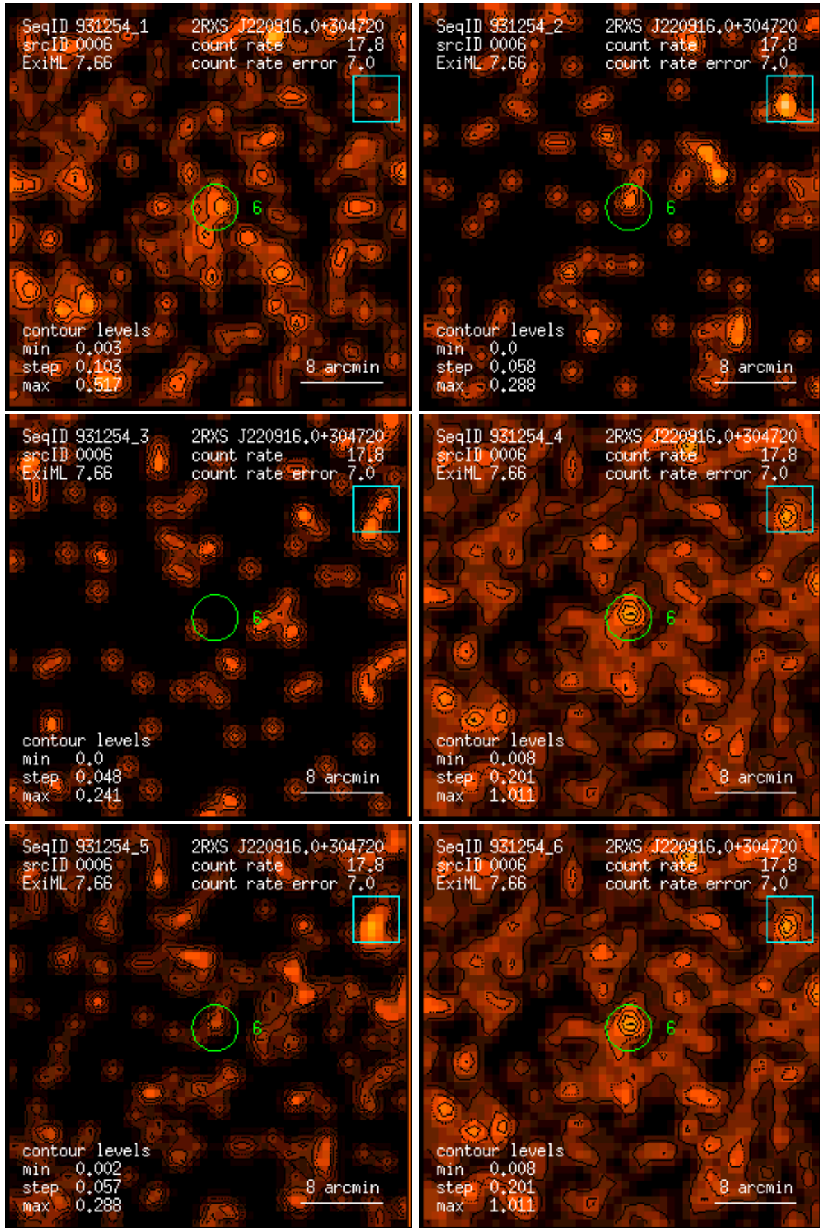
Figure 6: RASS 931254: detection 0006: band rate images, Gaussian filter: (1) PSPC channels 11 – 41, (2) 52 – 90, (3) 91 – 201, (4) 11 – 235, (5) 52 – 201, (6) 11 – 201. Broad band rates in counts/ks. Band rate contour levels in counts/ks/arcmin 2 .
