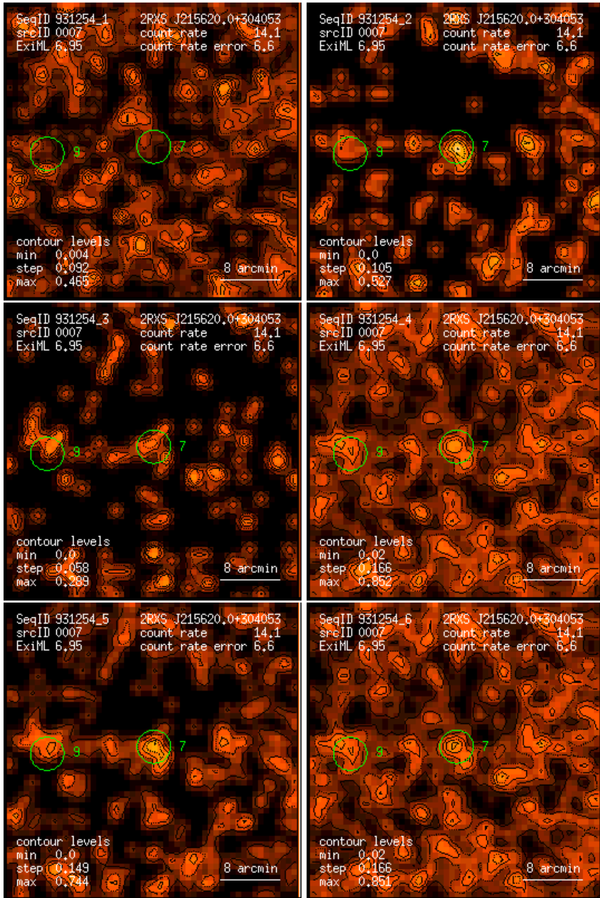
Figure 7: RASS 931254: detection 0007: band rate images, Gaussian filter: (1) PSPC channels 11 – 41, (2) 52 – 90, (3) 91 – 201, (4) 11 – 235, (5) 52 – 201, (6) 11 – 201. Broad band rates in counts/ks. Band rate contour levels in counts/ks/arcmin 2 .
