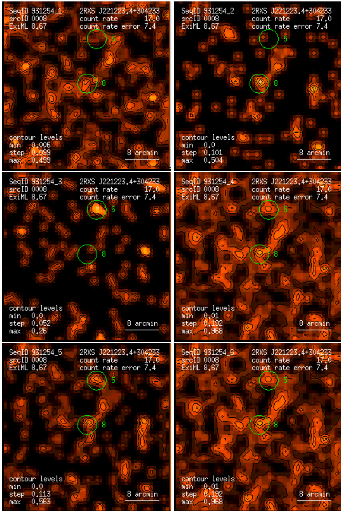
Figure 8: RASS 931254: detection 0008: band rate images, Gaussian filter: (1) PSPC channels 11 – 41, (2) 52 – 90, (3) 91 – 201, (4) 11 – 235, (5) 52 – 201, (6) 11 – 201. Broad band rates in counts/ks. Band rate contour levels in counts/ks/arcmin 2 .
