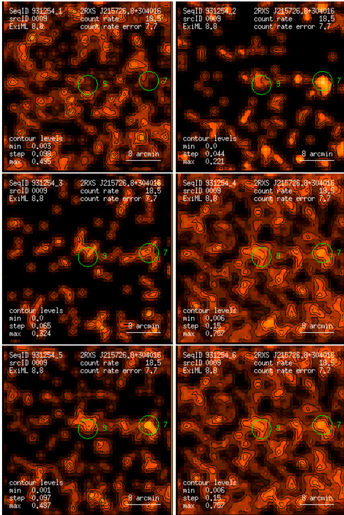
Figure 9: RASS 931254: detection 0009: band rate images, Gaussian filter: (1) PSPC channels 11 – 41, (2) 52 – 90, (3) 91 – 201, (4) 11 – 235, (5) 52 – 201, (6) 11 – 201. Broad band rates in counts/ks. Band rate contour levels in counts/ks/arcmin 2 .
