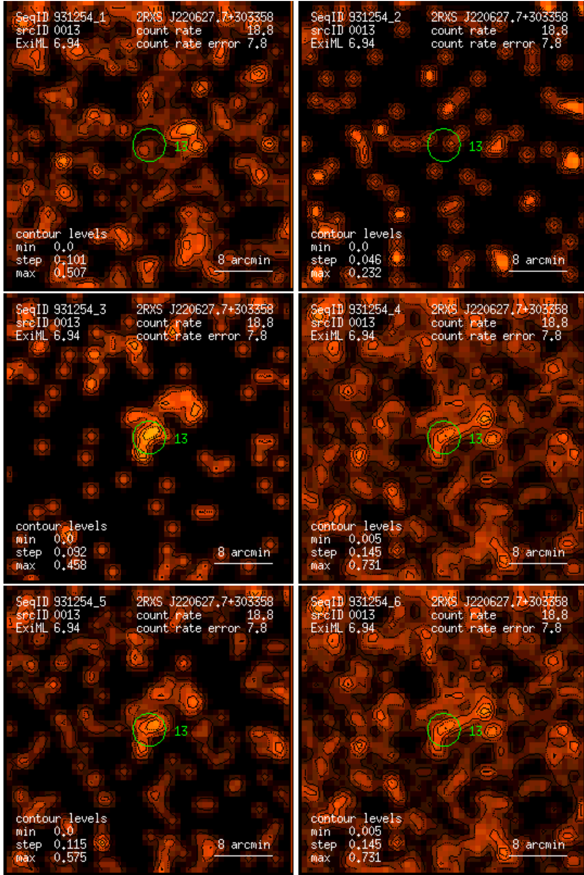
Figure 13: RASS 931254: detection 0013: band rate images, Gaussian filter: (1) PSPC channels 11 – 41, (2) 52 – 90, (3) 91 – 201, (4) 11 – 235, (5) 52 – 201, (6) 11 – 201. Broad band rates in counts/ks. Band rate contour levels in counts/ks/arcmin 2 .
